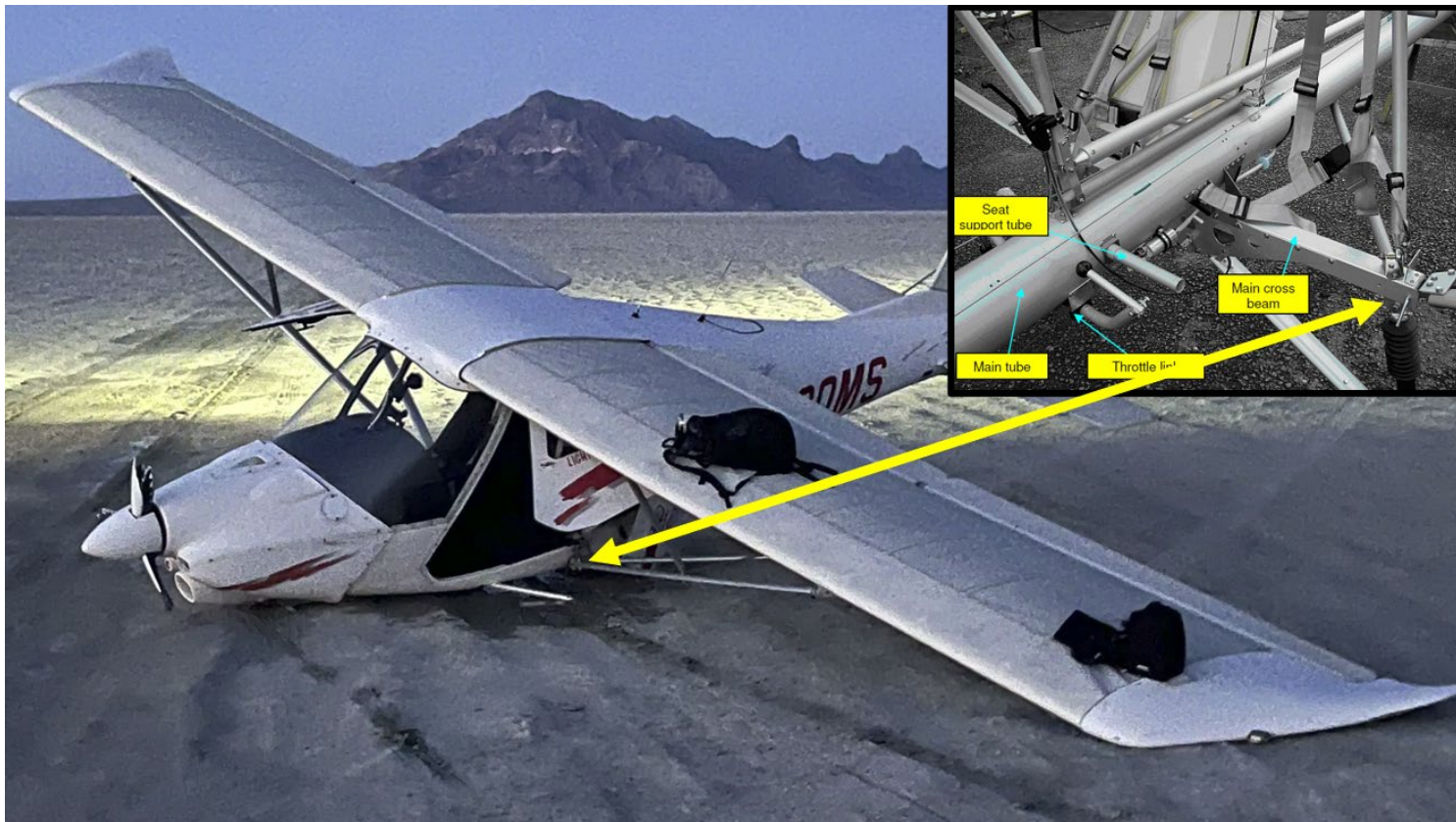
Photograph 1 - View of damage to the left main landing gear attachment points (Courtesy of LEA)
