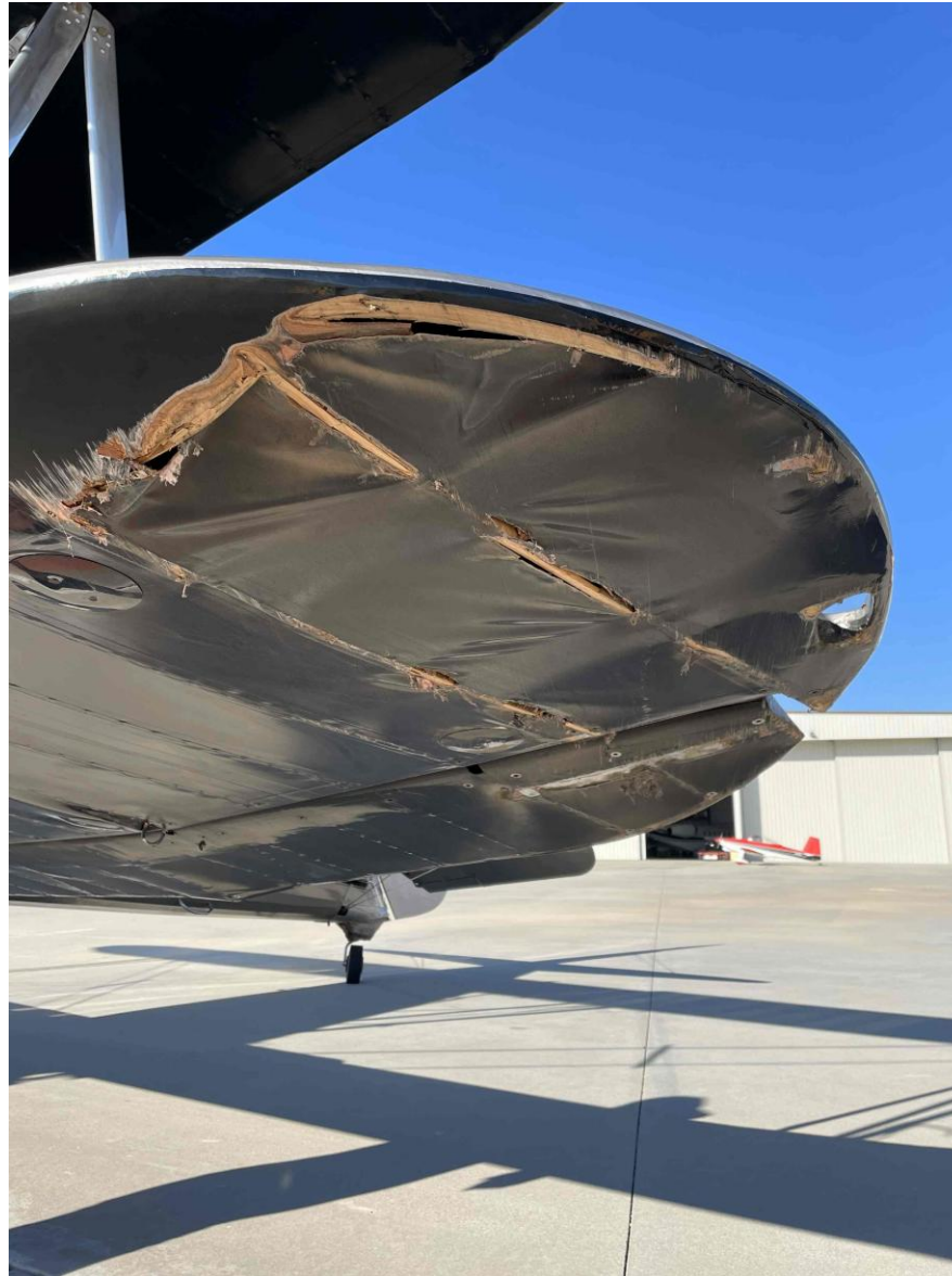
Photograph 1 - Lower left wing/aileron damage (Courtesy of KSEE Airport Ops)
