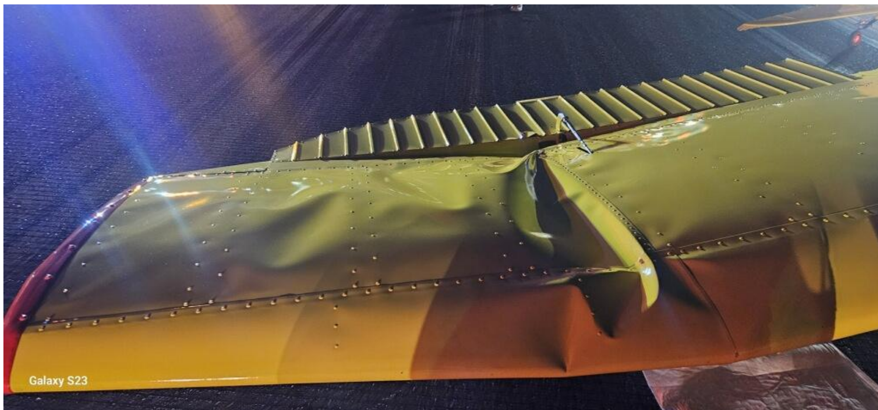
Photograph 2 - Aircraft Damage - Right Wing (Courtesy of Fresno Airport Operations)
