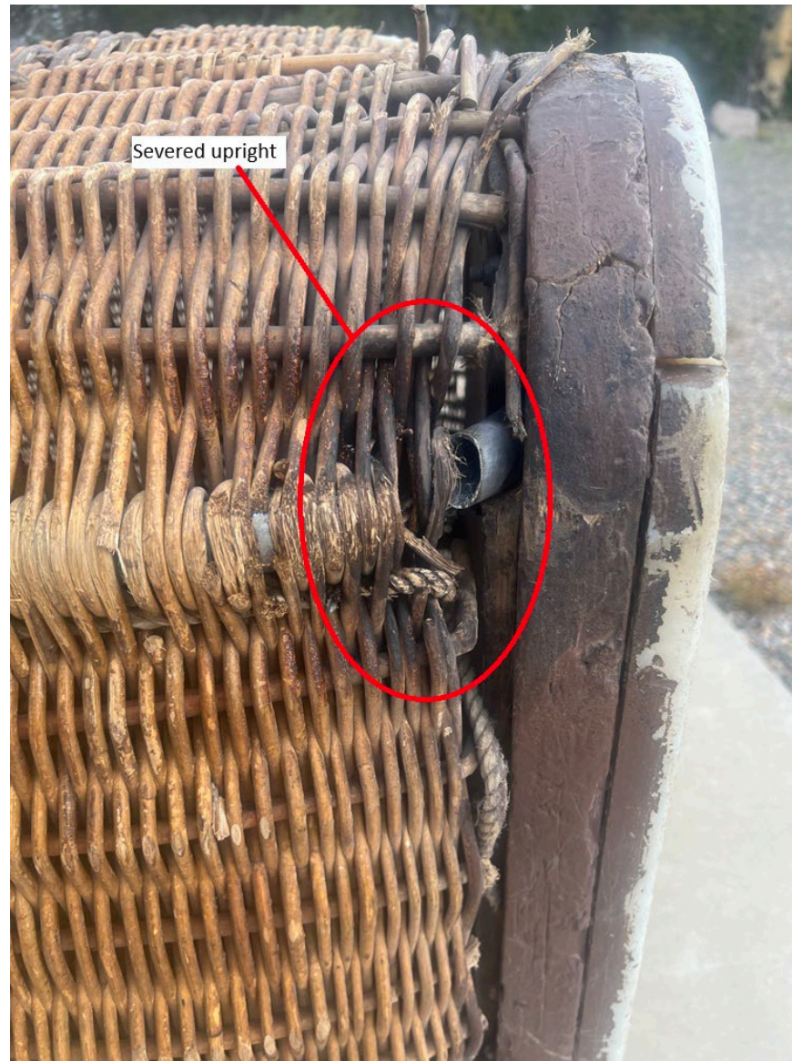
Photograph 2 - View of severed upright tube (Courtesy of Pilot)
