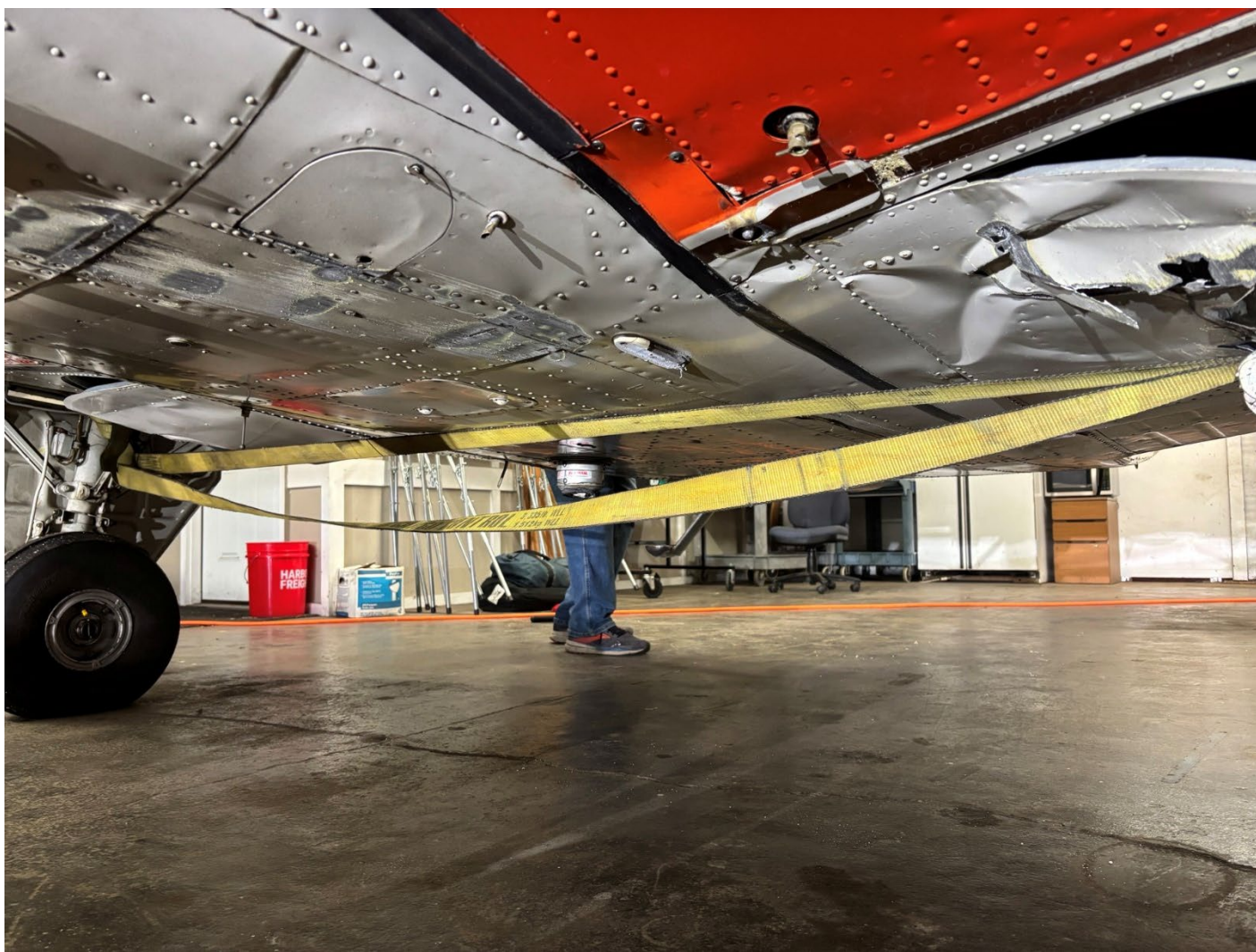
Photograph 1 - Bottom of left wing damage (Courtesy of pilot)
