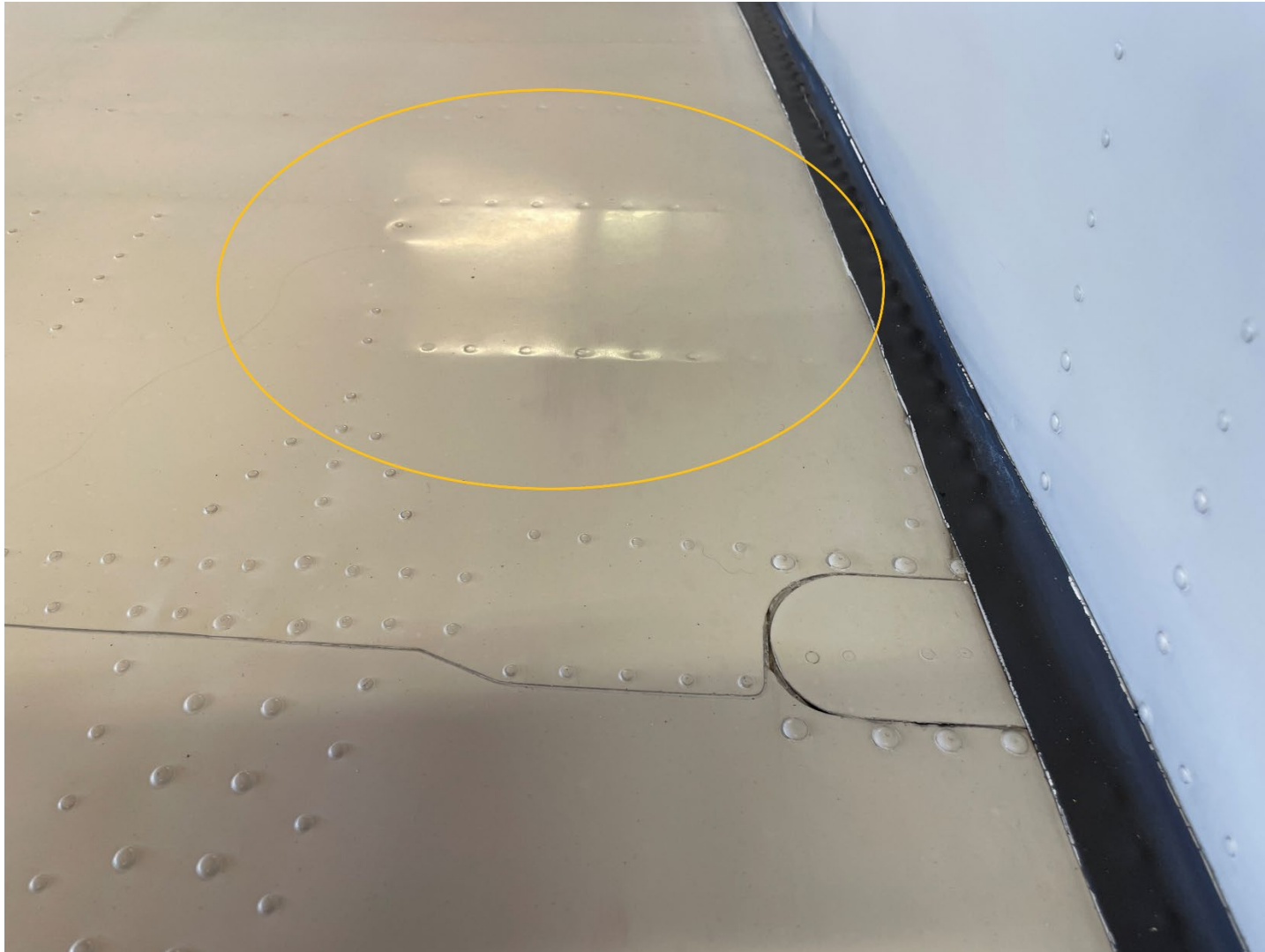
Photograph 3 - Raised rivets indicating internal left wing damage (Courtesy of maintenance)
