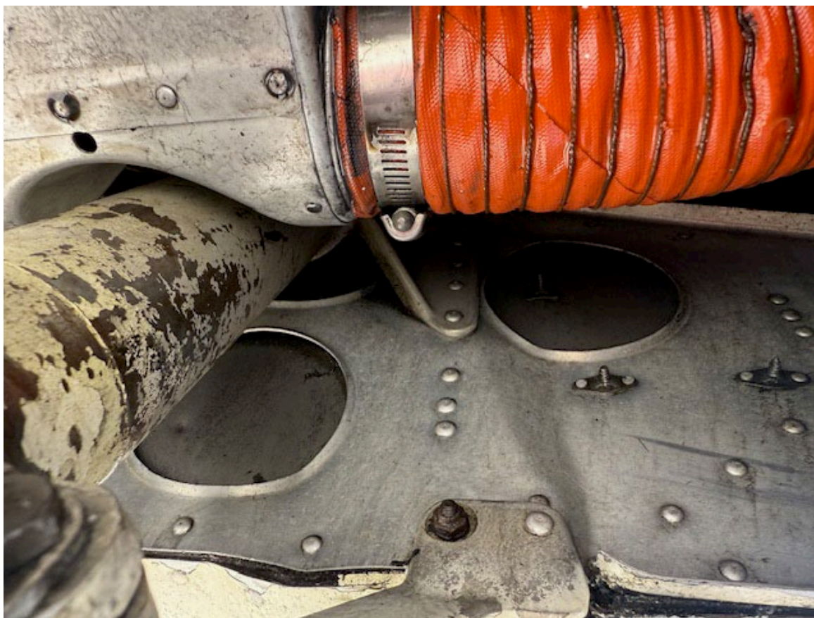
Photograph 1 - Substantial damage to firewall. (Courtesy of the airport manager)
