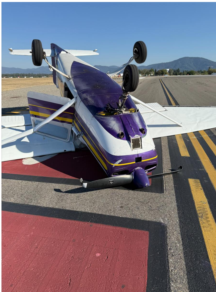
Photograph 1 - Aircraft Final Position and Damage (via COE airport ops)
