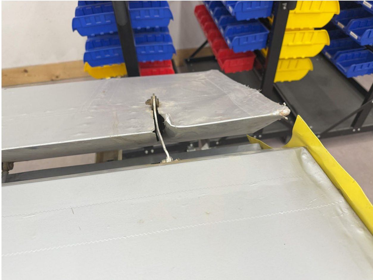
Photo 3 - View of damage to outboard right aileron and attachment point (Courtesy of A&P)
