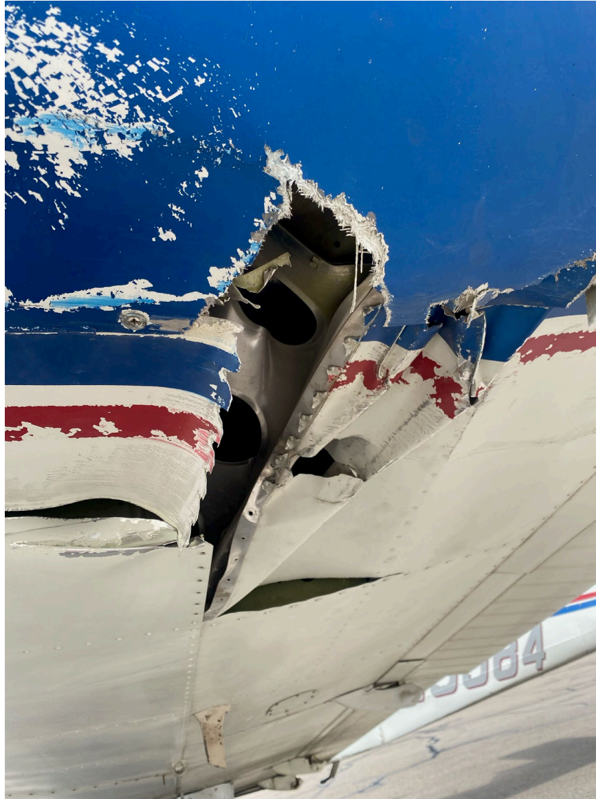
Photograph 2 - Closeup view of underside of left wing (Courtesy of Pilot)
