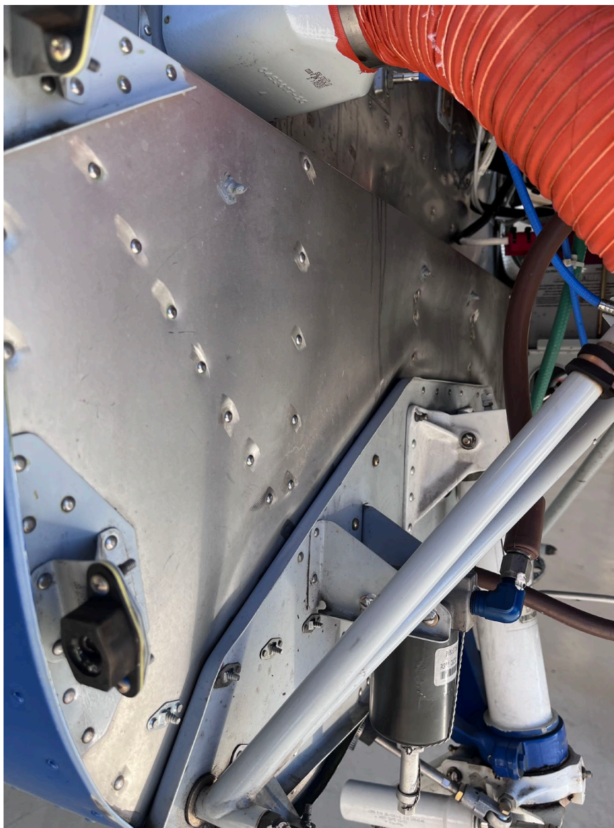
Photograph 3 - Firewall damage (Courtesy of ERAU)
