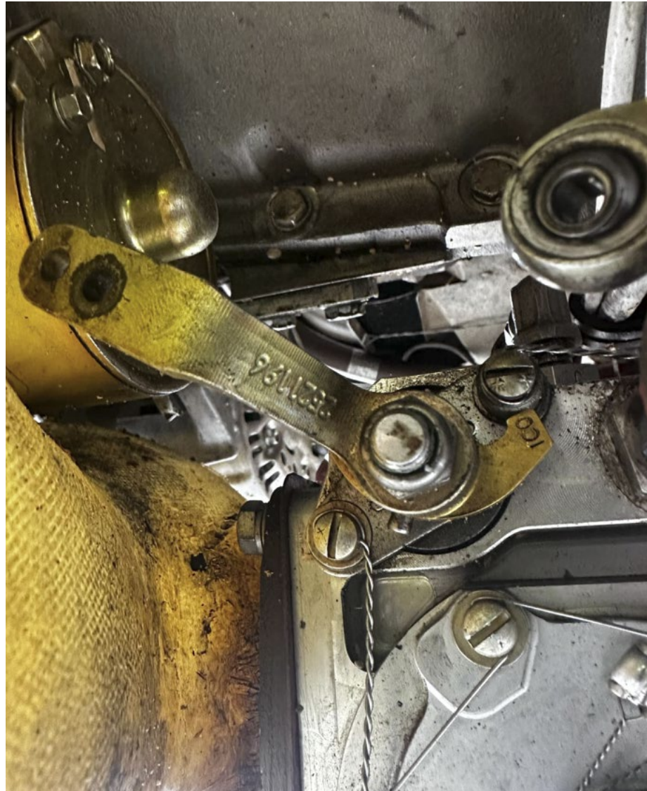
Photograph 2 - View of the mixture control arm and the bellcrank rod end bearing, absent the connecting bolt, washers and castellated nut (Courtesy of Aircraft Recovery)
