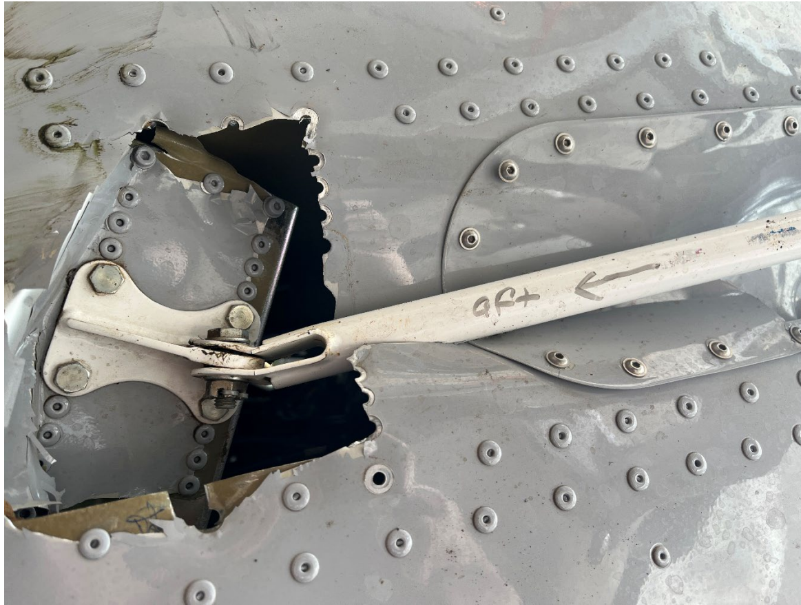
Photograph 6 - Damage to gear strut. (Courtesy of FAA)
