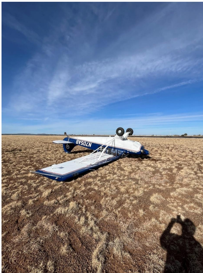
Photograph 2 - Accident site, view of the left forward side of the airplane. (Courtesy of Airport Operations)
