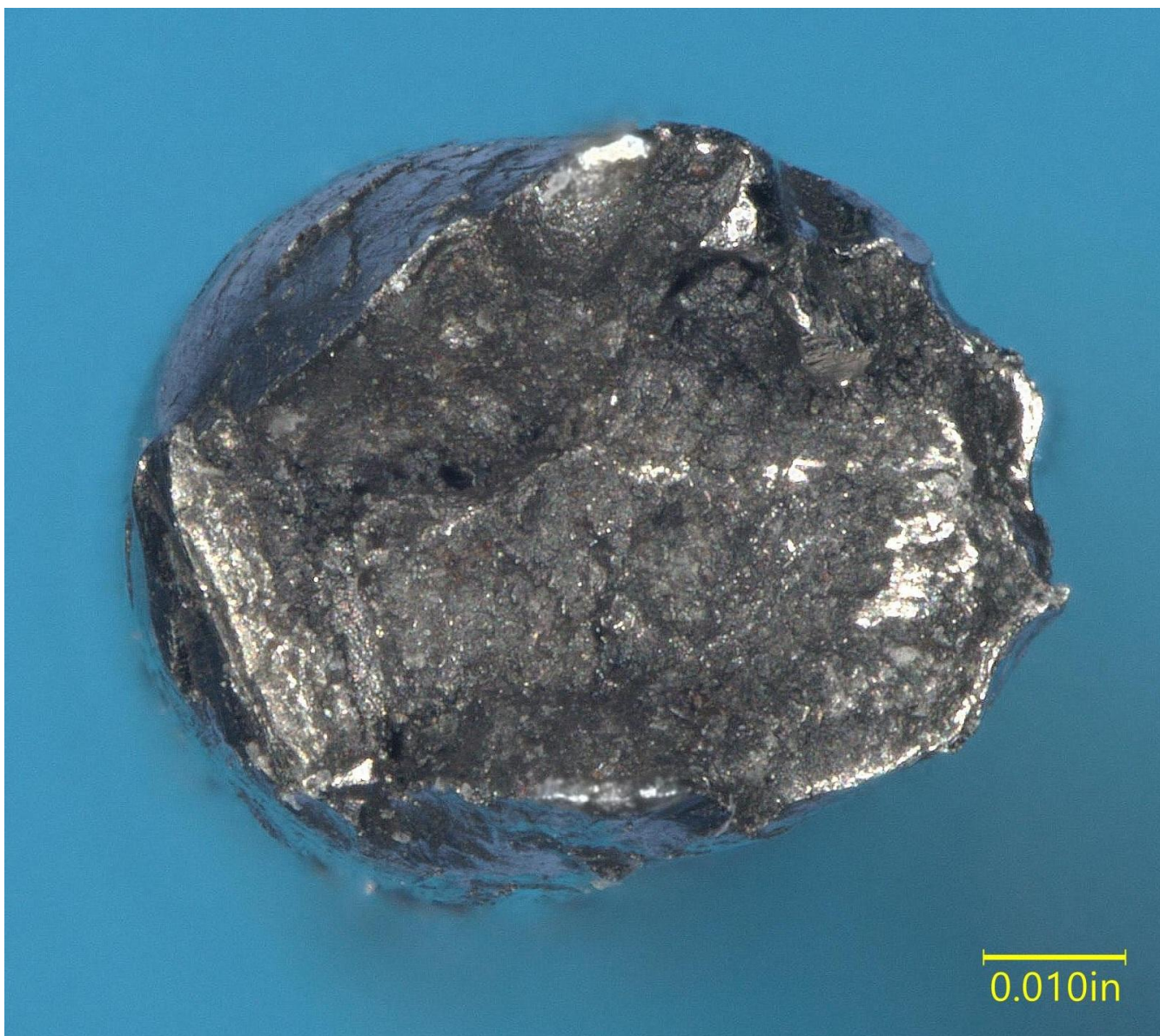
Photograph 3 - Wire fracture surface (80x)
