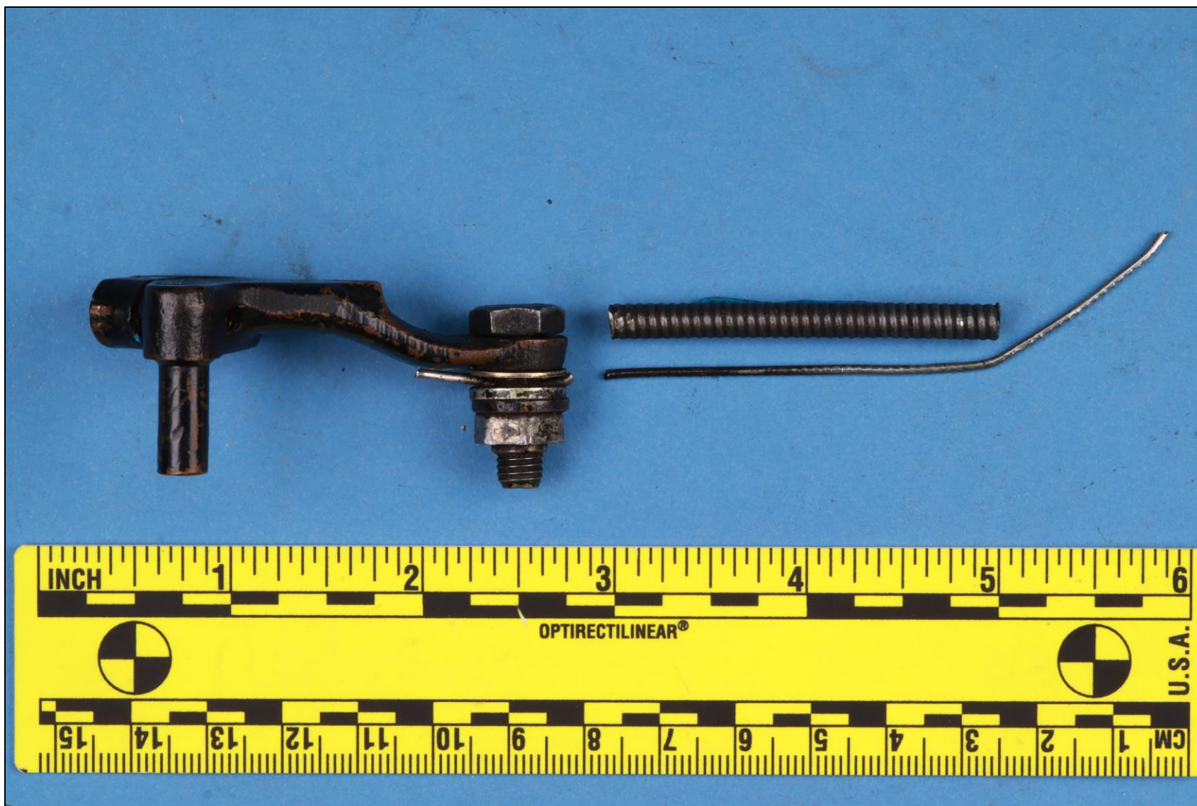
Photograph 1 - Mixture cable, overall.
