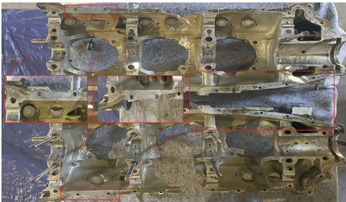
Photograph 5 - Internal view of left and right engine case halves, highlighting fretting to forward section of each case half (Courtesy of NTSB)
