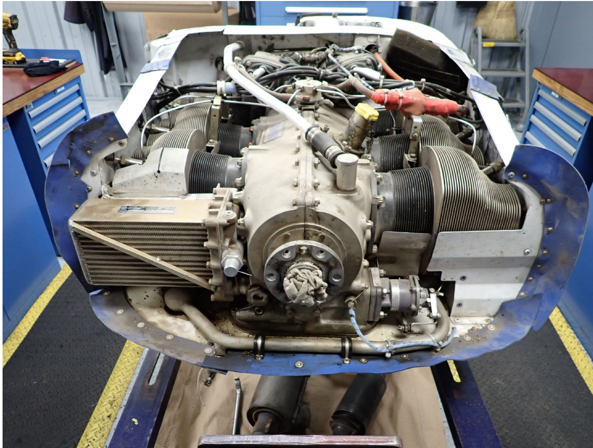
Photograph 3 - Engine mounted on exam stand.
