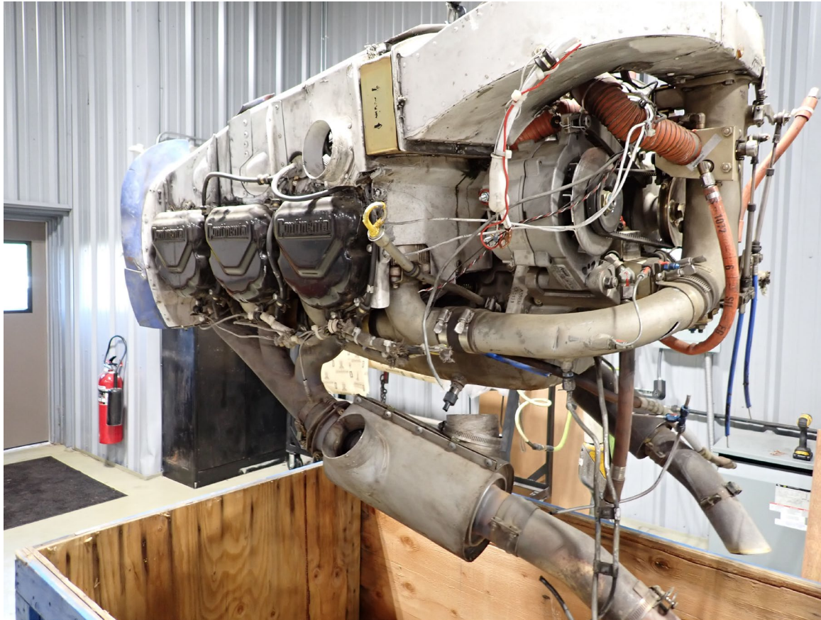
Photograph 2 - Engine removal from crate.
