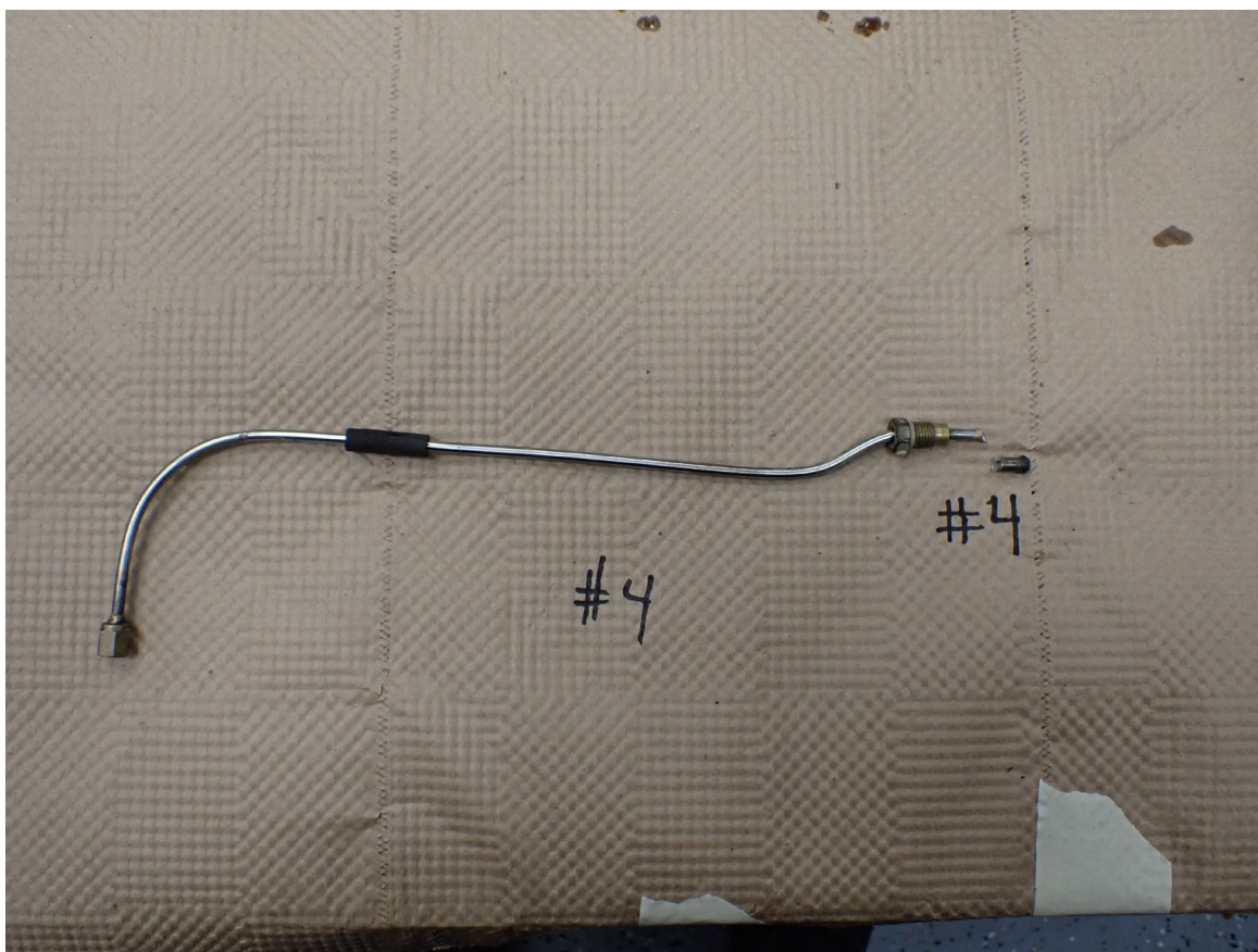
Photograph 4 - Cylinder number 4 fuel injection assembly tube.
