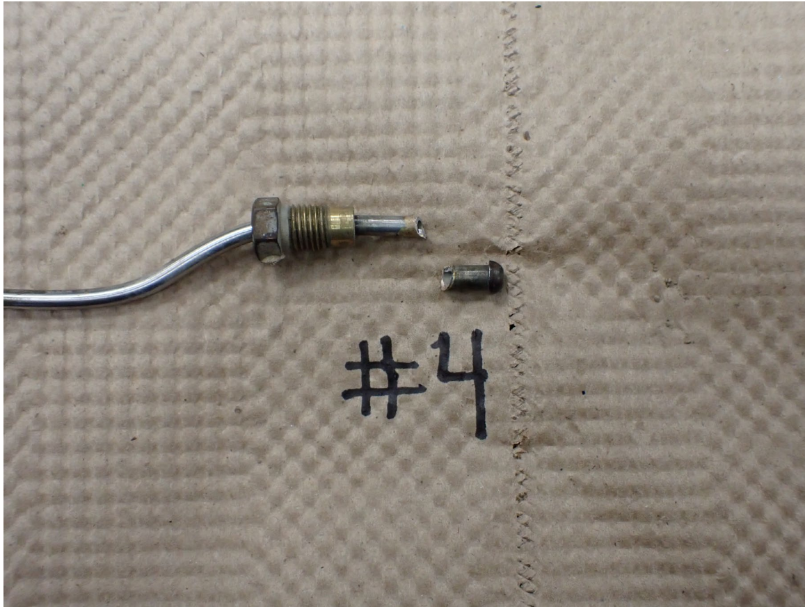
Photograph 5 - Cylinder number 4 fuel injection assembly tube.
