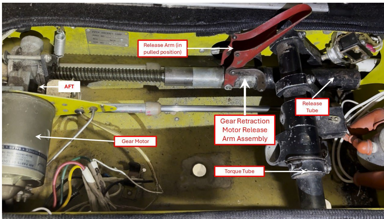
Photograph 4 - View of manual release assembly, gear motor, and torque tube
