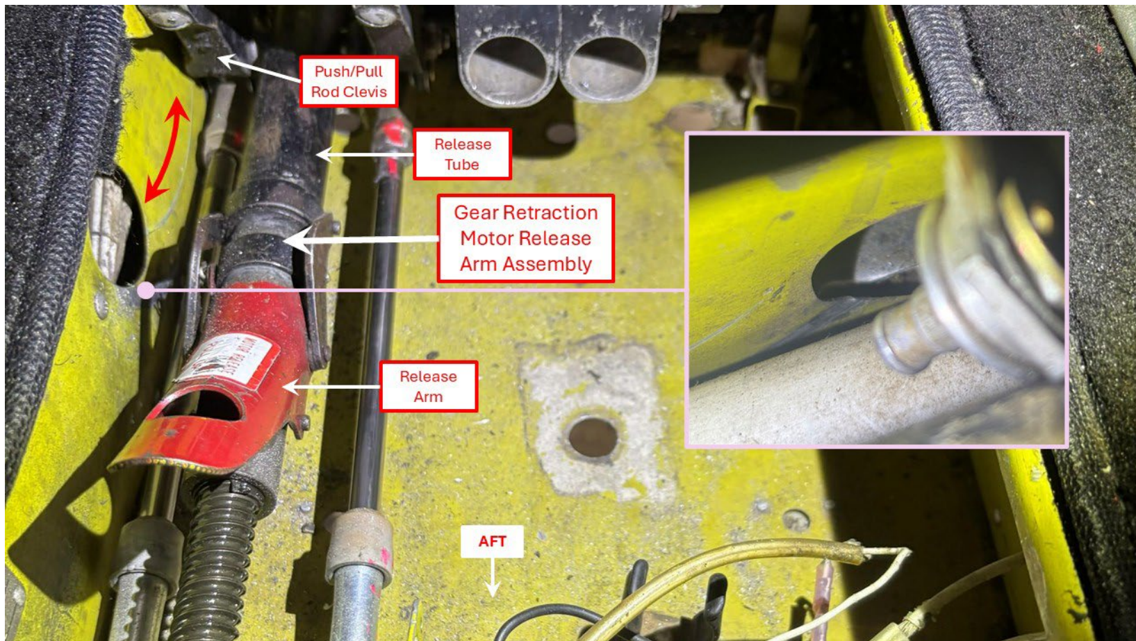
Photograph 5 - Manual release assembly housing and damage to side structure inhibiting movement of torque tube
