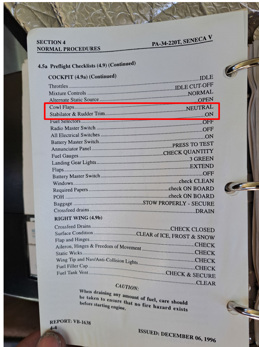
Photograph 6 - View of POH preflight check list
