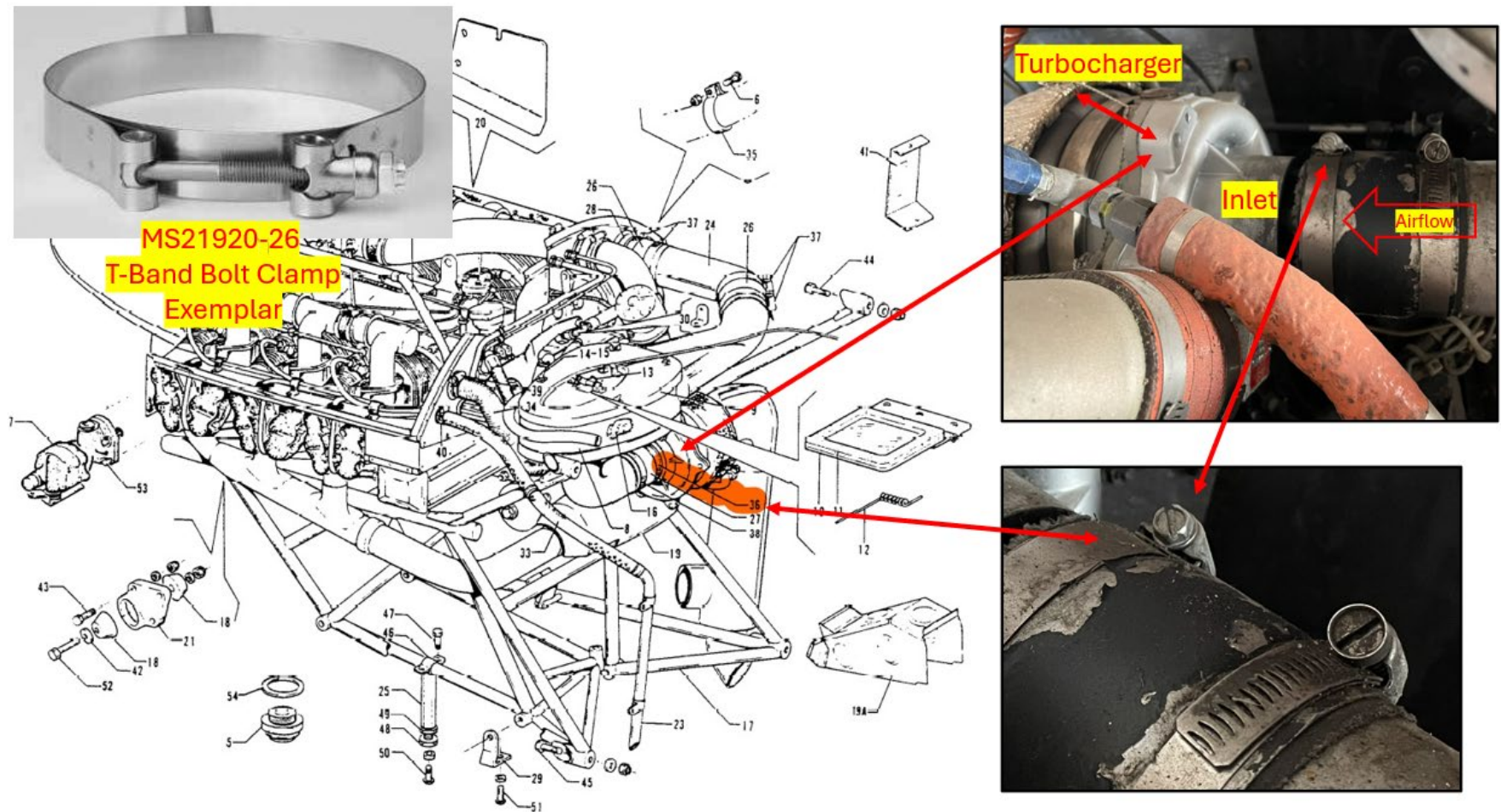
Photograph 3 - View of IPC excerpt with turbocharger, inlet house, and t-band clamp exemplar photo overlays
