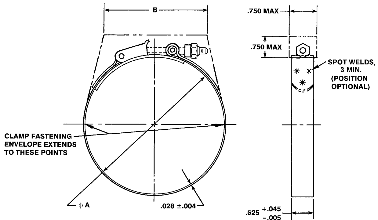
FIGURE 1. Hose clamp.
