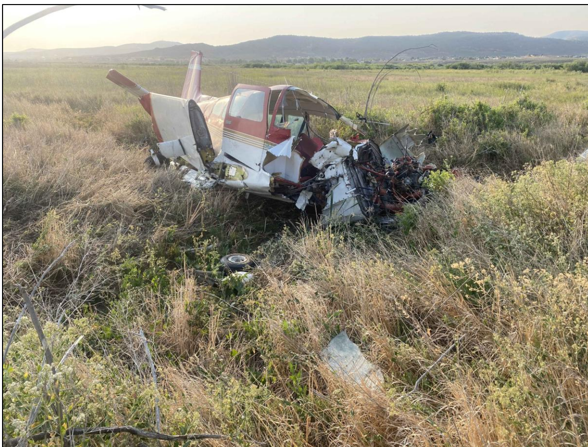
Photograph 1 - Accident site, fwd right view of the main wreckage. (Courtesy of Airport Ops)
