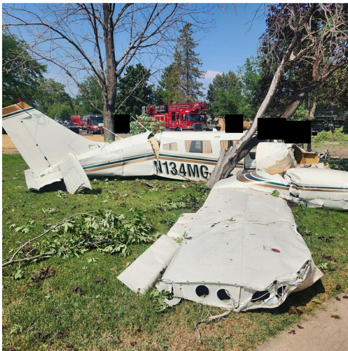
Photograph 2 - Right Side View of Airplane (Courtesy of Law Enforcement)
