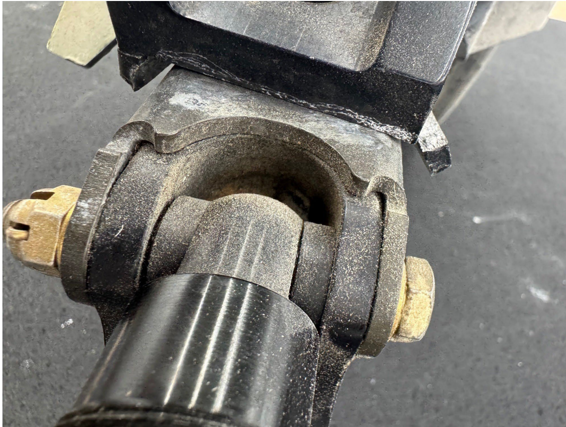
Photograph 6 - Tailwheel Assembly Damage Closeup (Courtesy of Pilot)
