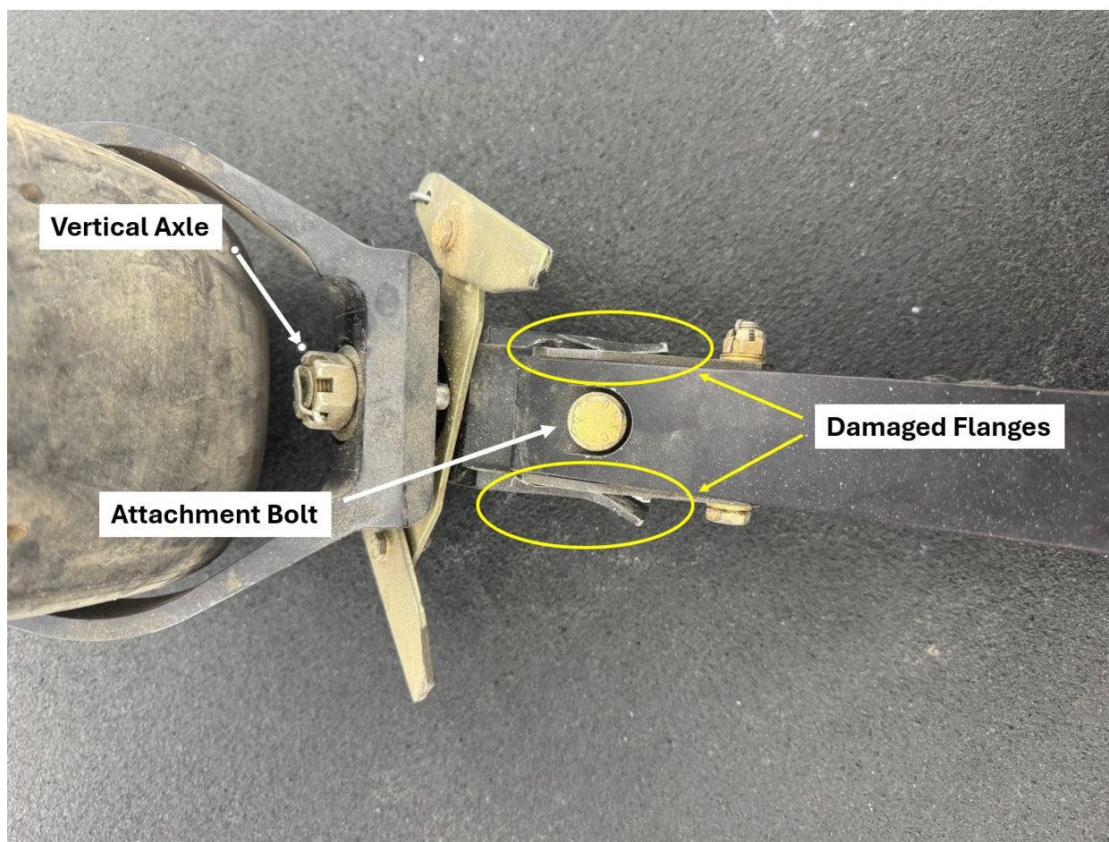
Photograph 5 - Tailwheel Assembly Damage (Courtesy of Pilot)
