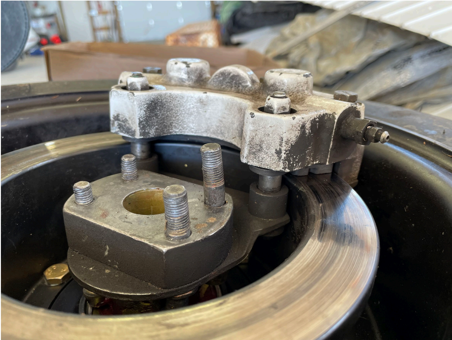
Photograph 2 - View of wheel assembly
