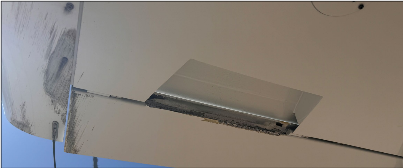
Photograph 1 - Airplane's right aileron (counterbalance-weight separated) as viewed from the bottom. (Courtesy of FAA)
