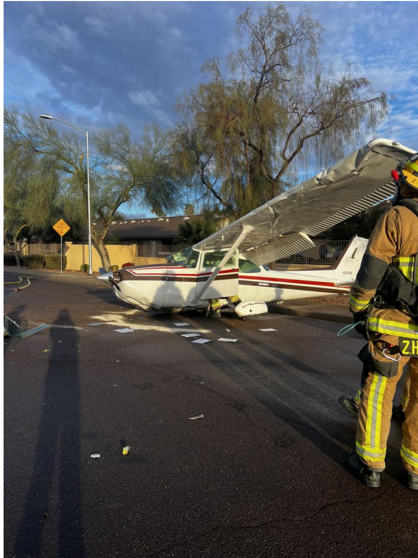
Photograph 1 - Accident site, main wreckage. (Courtesy of the FAA)
