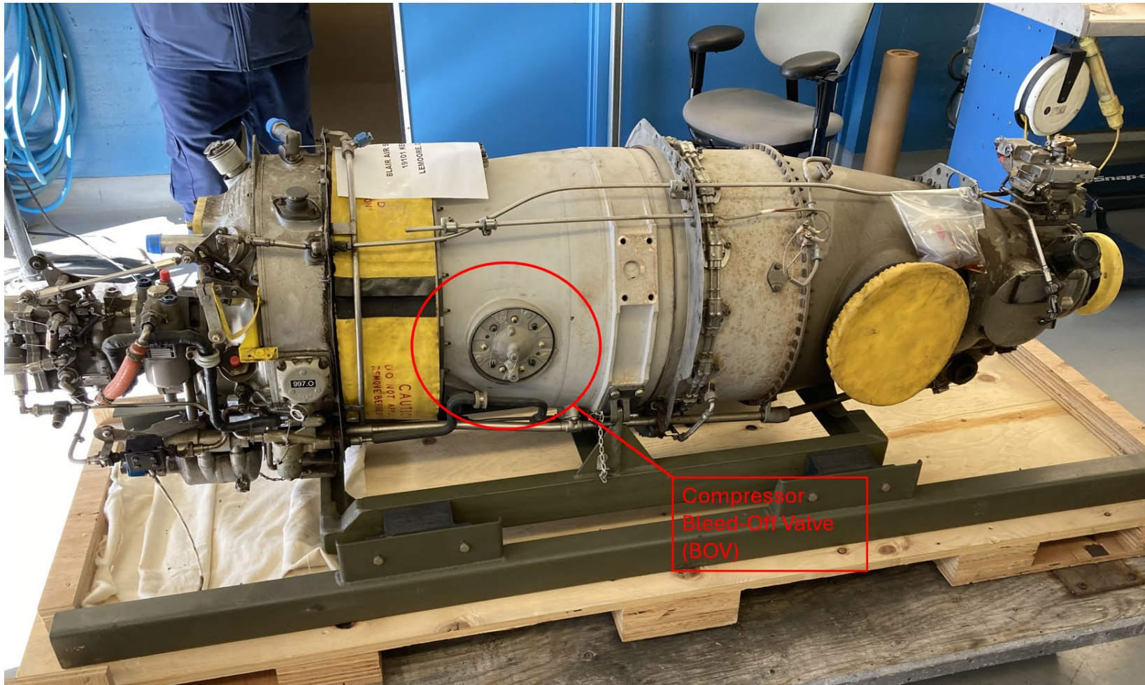
Photograph 3 - Engine received with compressor bleed-off valve (BOV) center at PWC.
