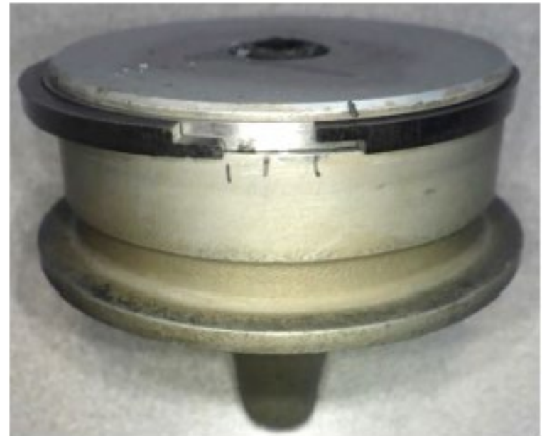
Photograph 6 - BOV piston removed from housing. (Courtesy of PWC)
