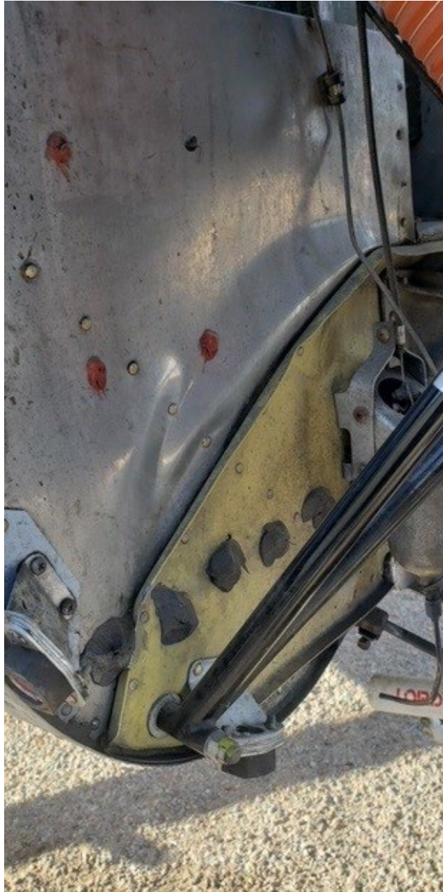
Photo 3 – Damage to engine firewall (courtesy of FAA)
