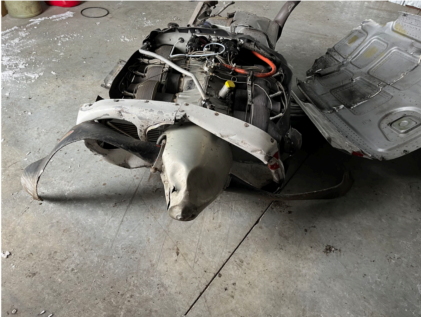
Photograph 3 - The right engine and propeller. (Courtesy of Textron Aviation.)
