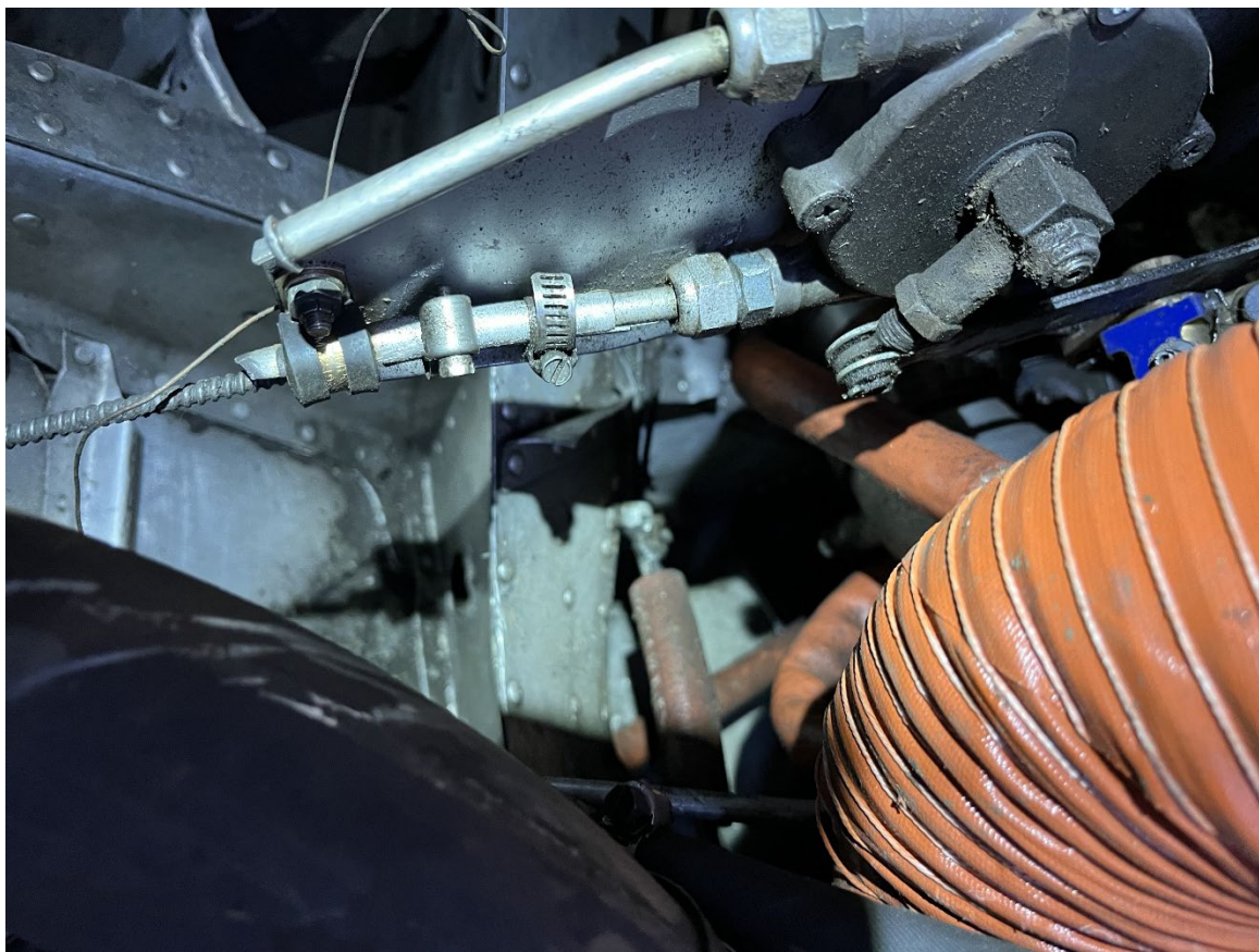
Photograph 4 - The left engine throttle control. (Courtesy of Textron Aviation.)
