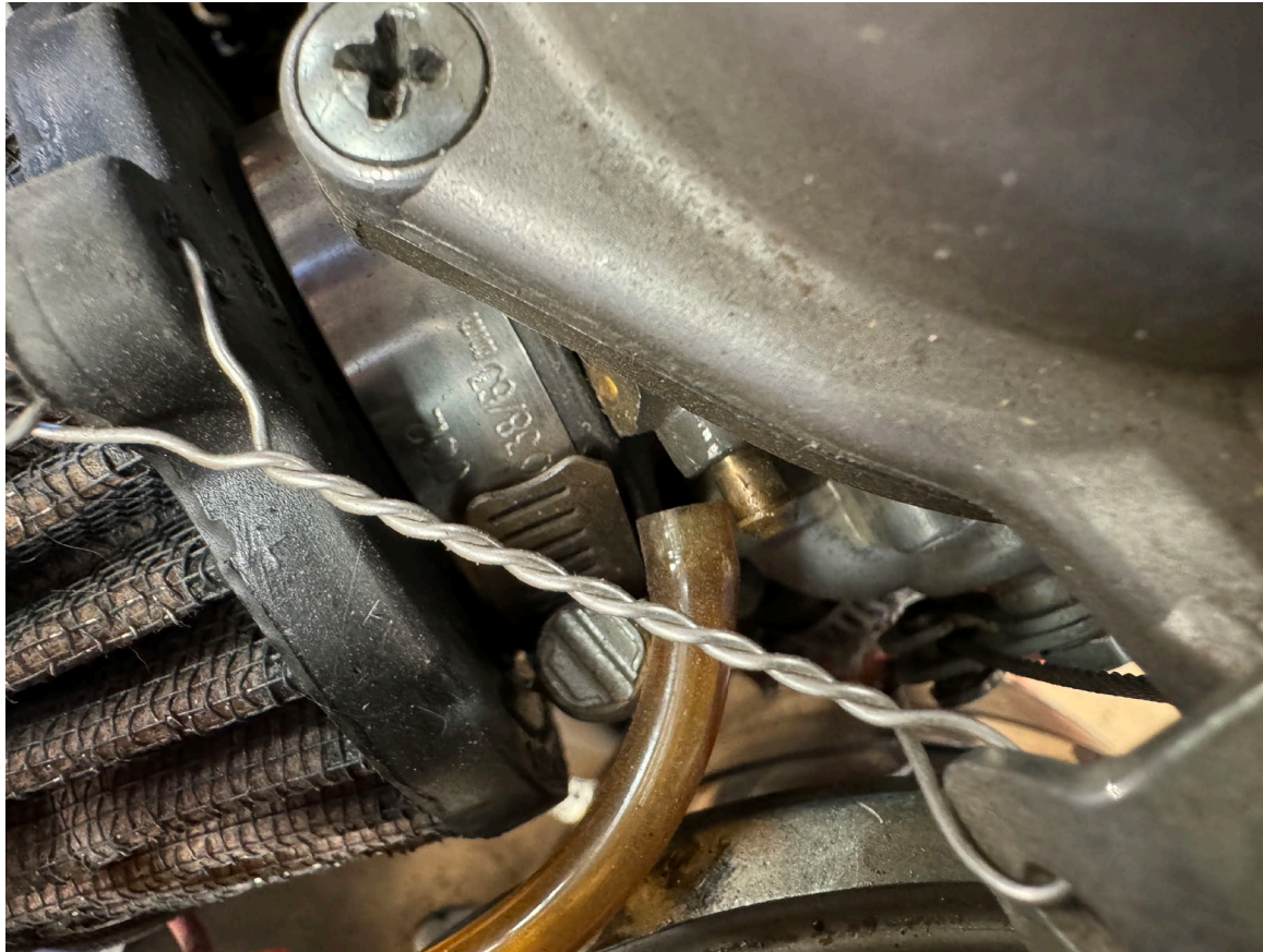
Photograph 2 - Disconnected carburetor float bowl vent line 1/3 side.
