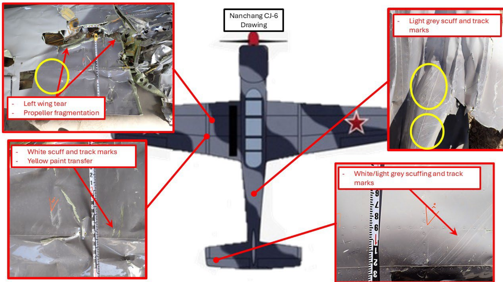
Photograph 10 - CJ-6A (N313YK) damage figure
