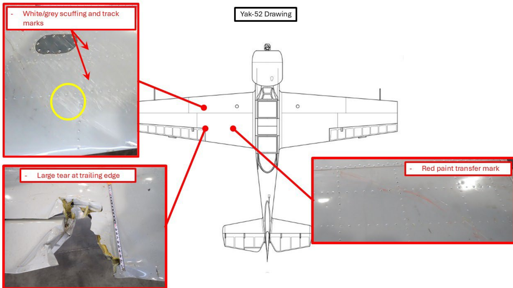
Photograph 11 - Yak 52 (N5287) damage figure
