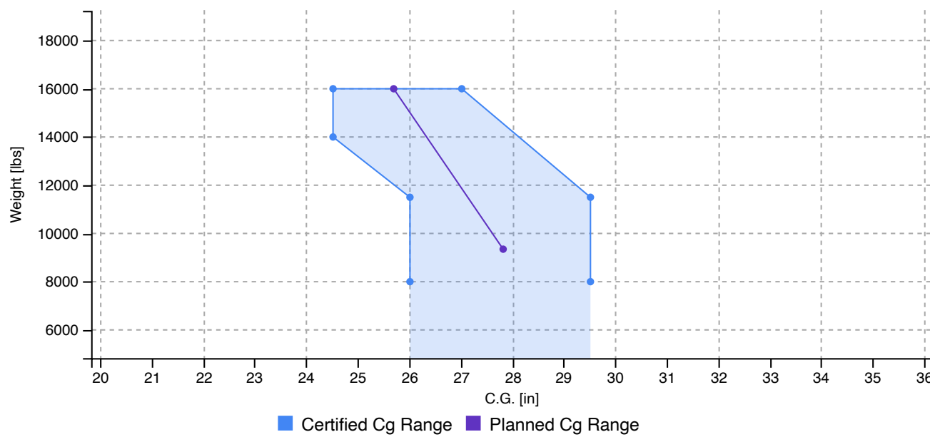
Weight and Balance Plot
