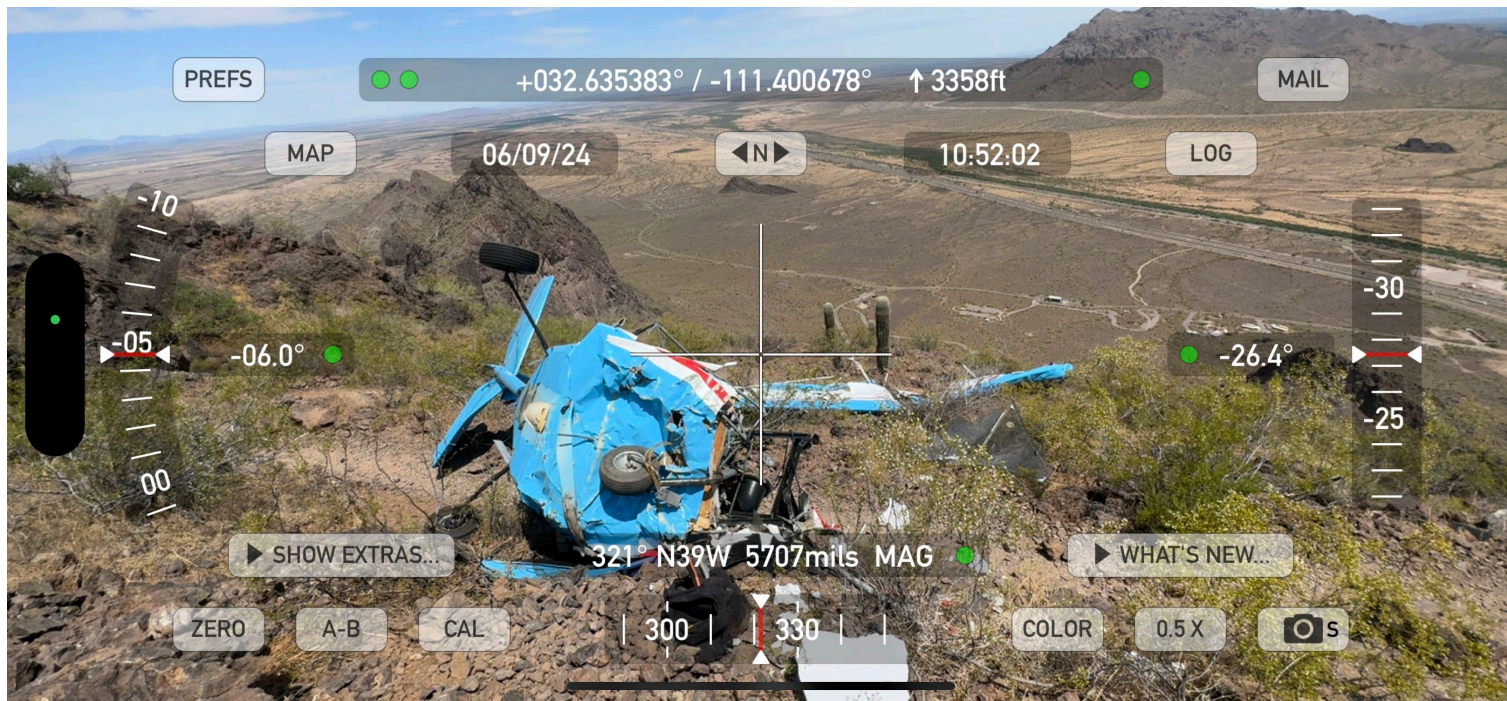
Photograph 6 - Southeast to northwest view of the wreckage and impact damage to lower fuselage and nose section
