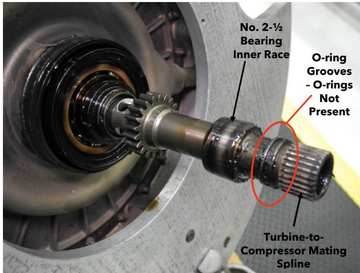
Photograph 3 - Turbine to Compressor Mating Spline
