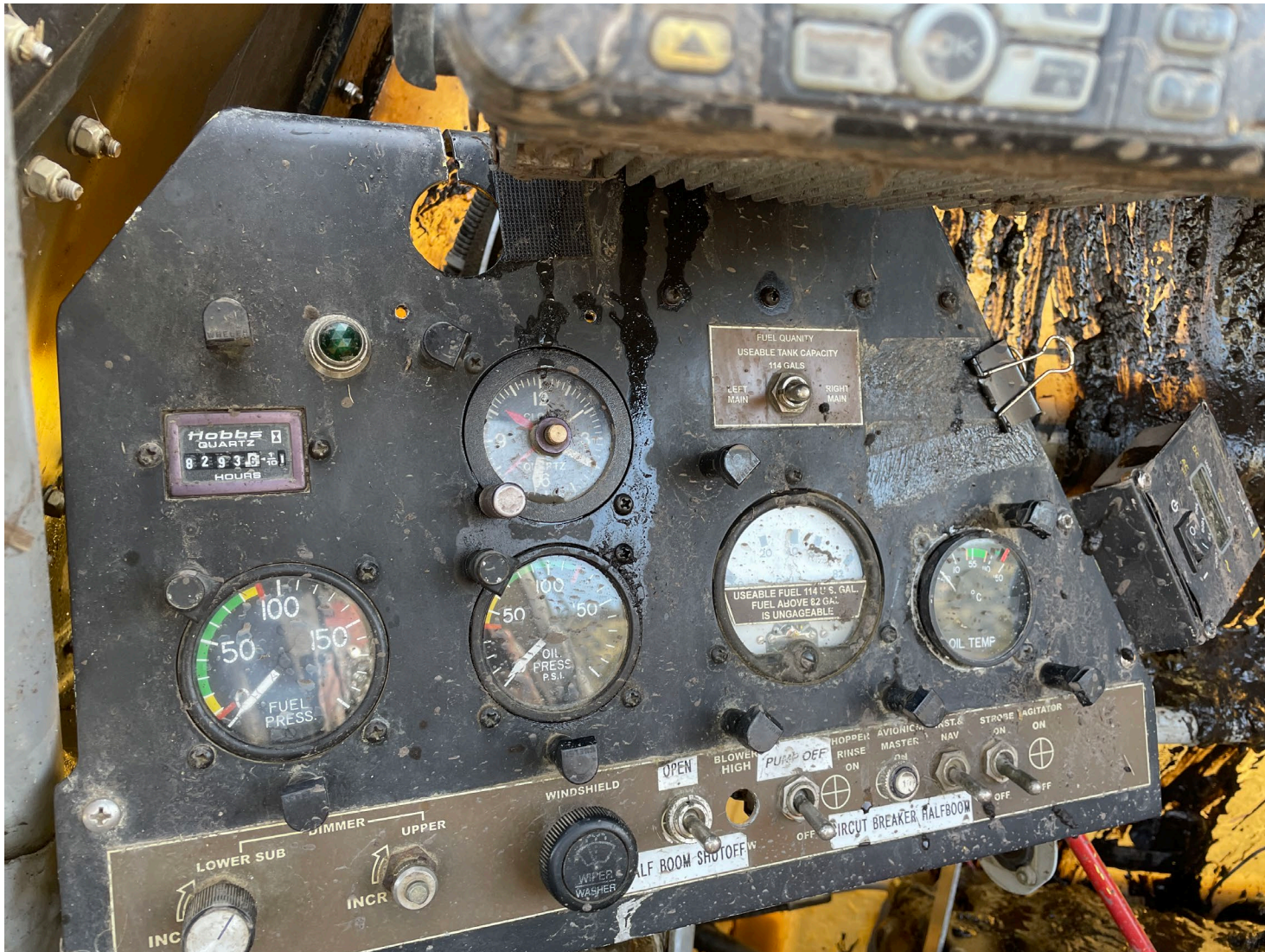
Photograph 2 - The fuel gauge and tank switch.
