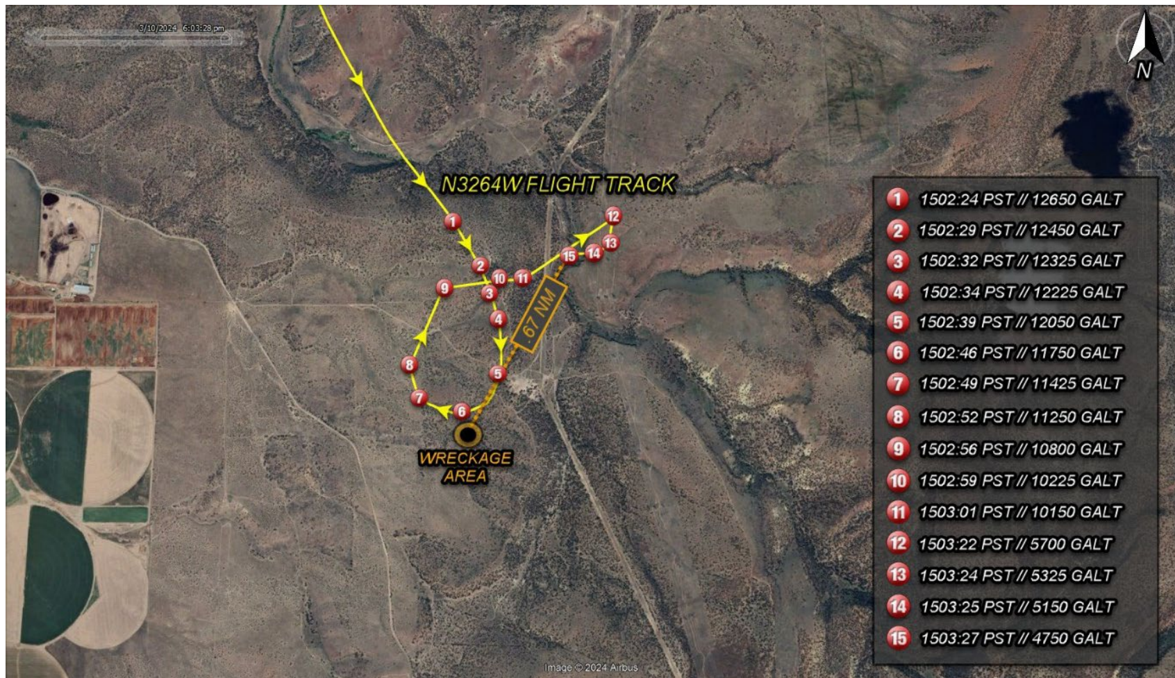
Photograph 1 - Southeast flight track to accident site
