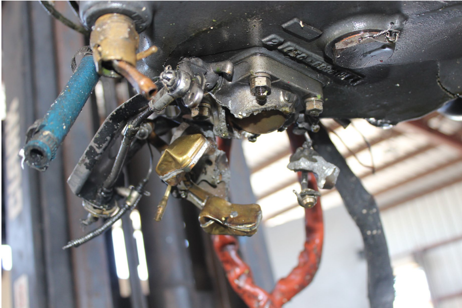
Photograph 5 - View of carburetor damage (Courtesy of Lycoming)
