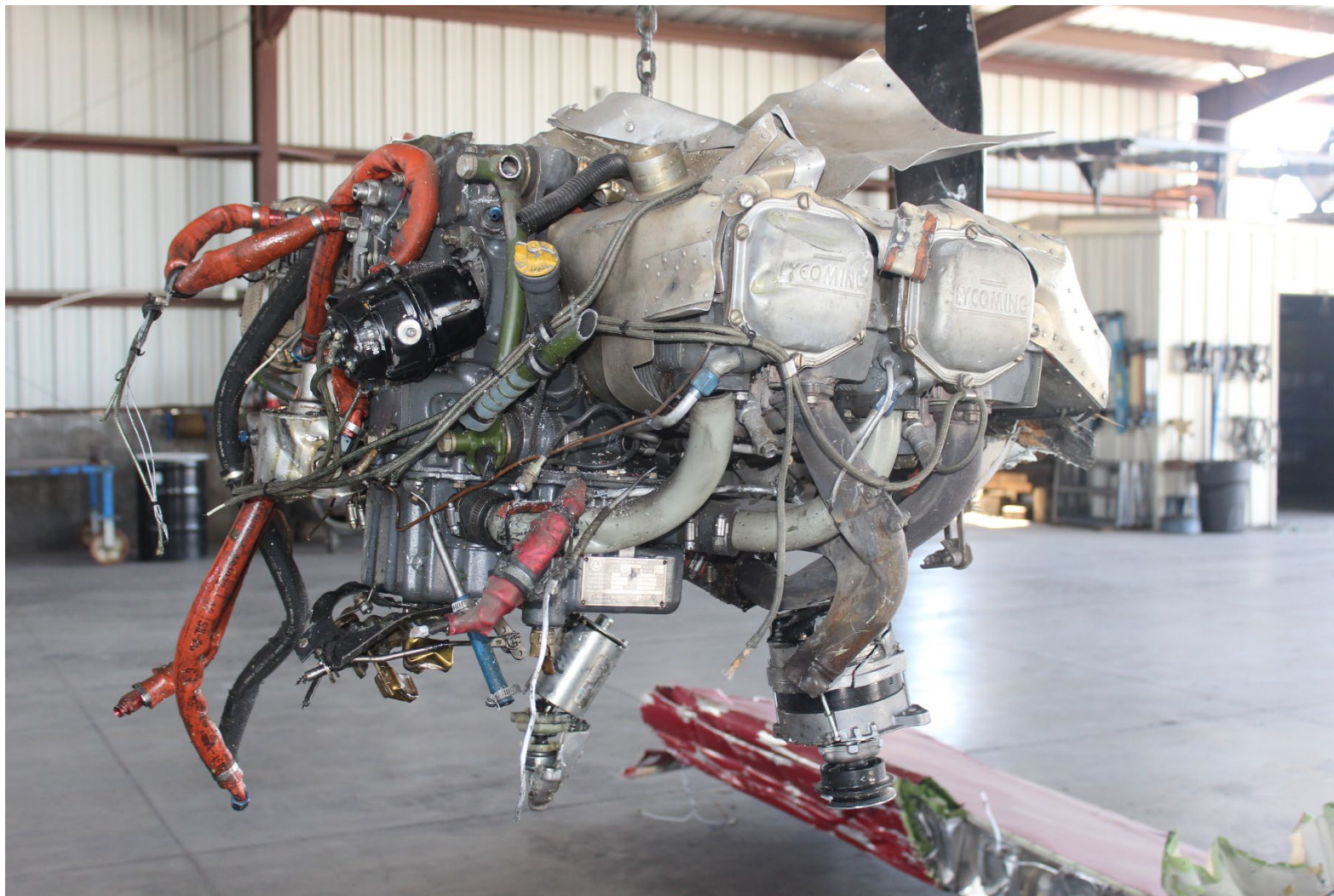
Photograph 4 - View of engine separated from airframe (Courtesy of Lycoming)
