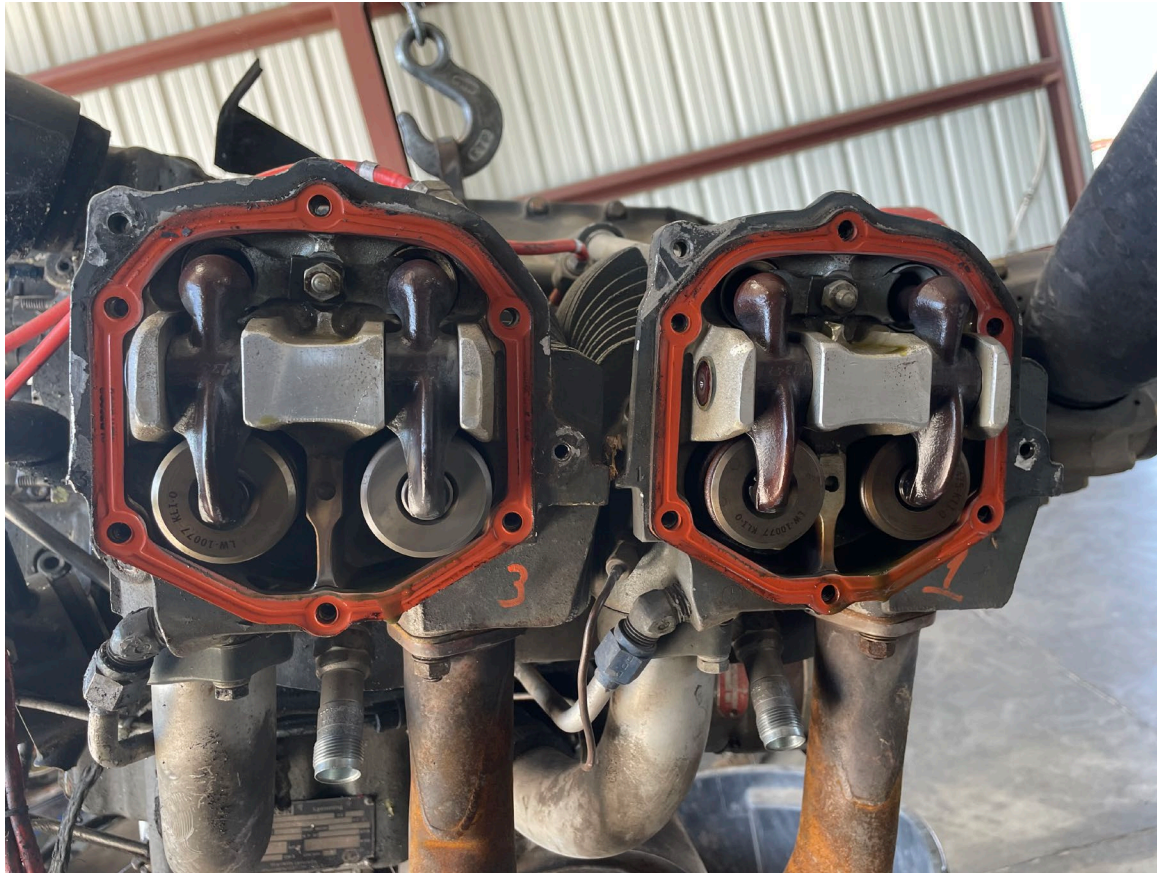
Photograph 7 - View of no. 1 & 3 cylinders
