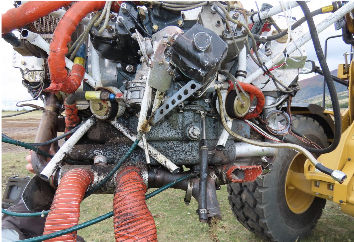
Photograph 4 -Engine oil saturation throughout lower accessory case
