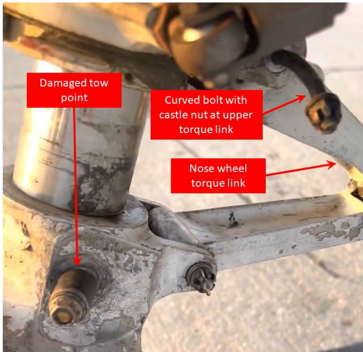
Photo 3 – Nose landing gear strut and torque link after pickup truck collision (still from video courtesy of airplane owner)
