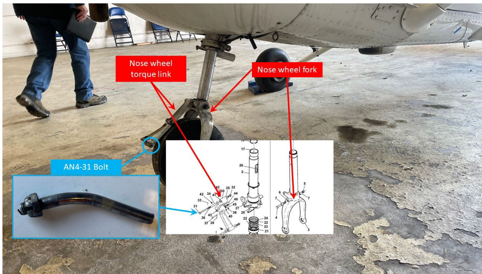
Photo 2 – Figure of fractured bolt and nose landing gear torque link (photo courtesy of FAA)
