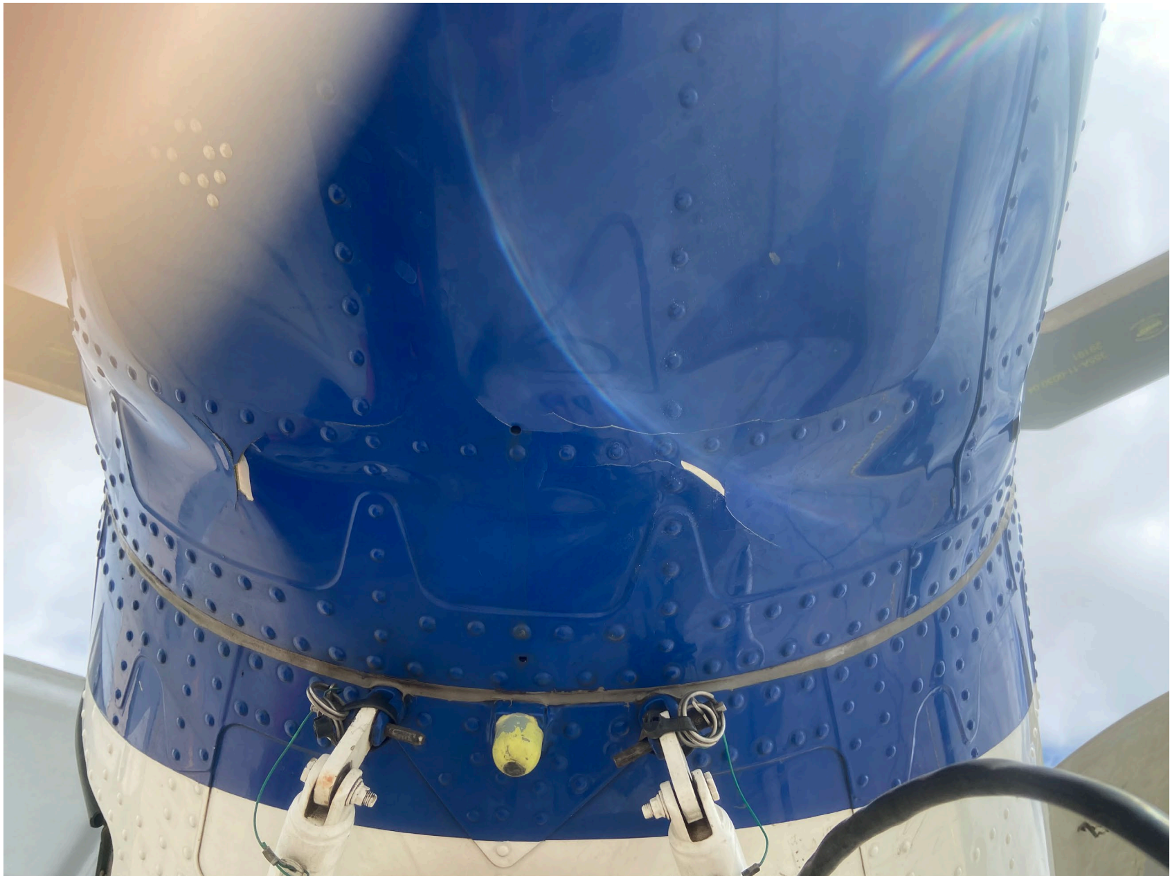
Photo 2 – Bottom damage tail boom (Photo courtesy of Customs and Border Protection)
