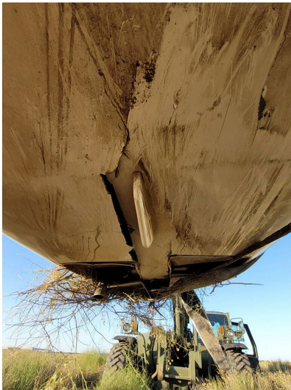
Photo 2 – Bottom view (Photo courtesy of pilot)
