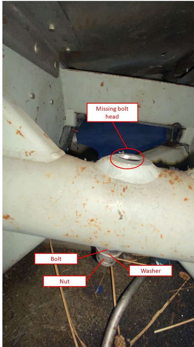
Photo 6 – Right main landing gear support assembly with fractured bolt (courtesy of FAA)
