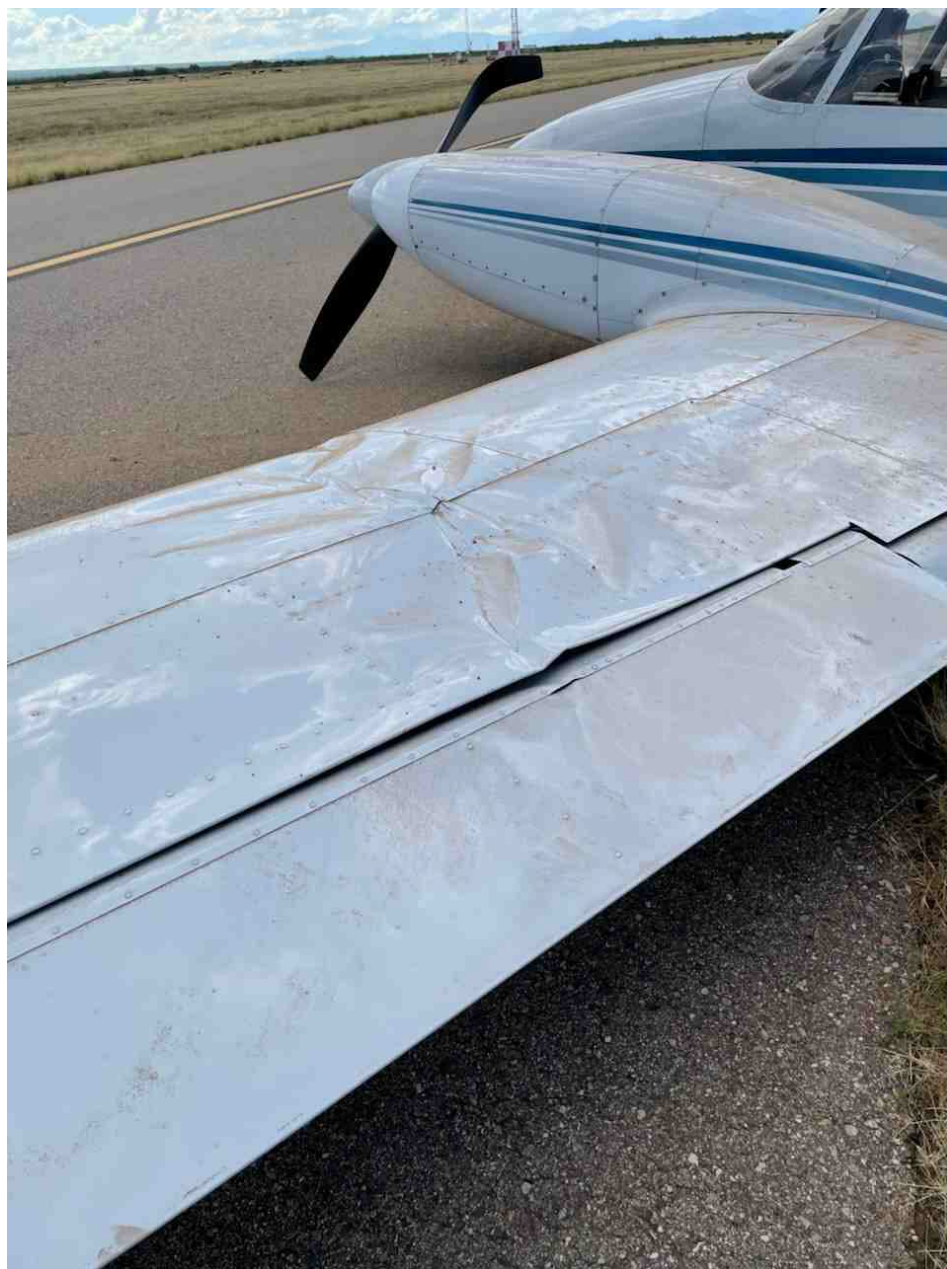
Photo 2 – Left Wing Damage (AZ Aerotech Photo)
