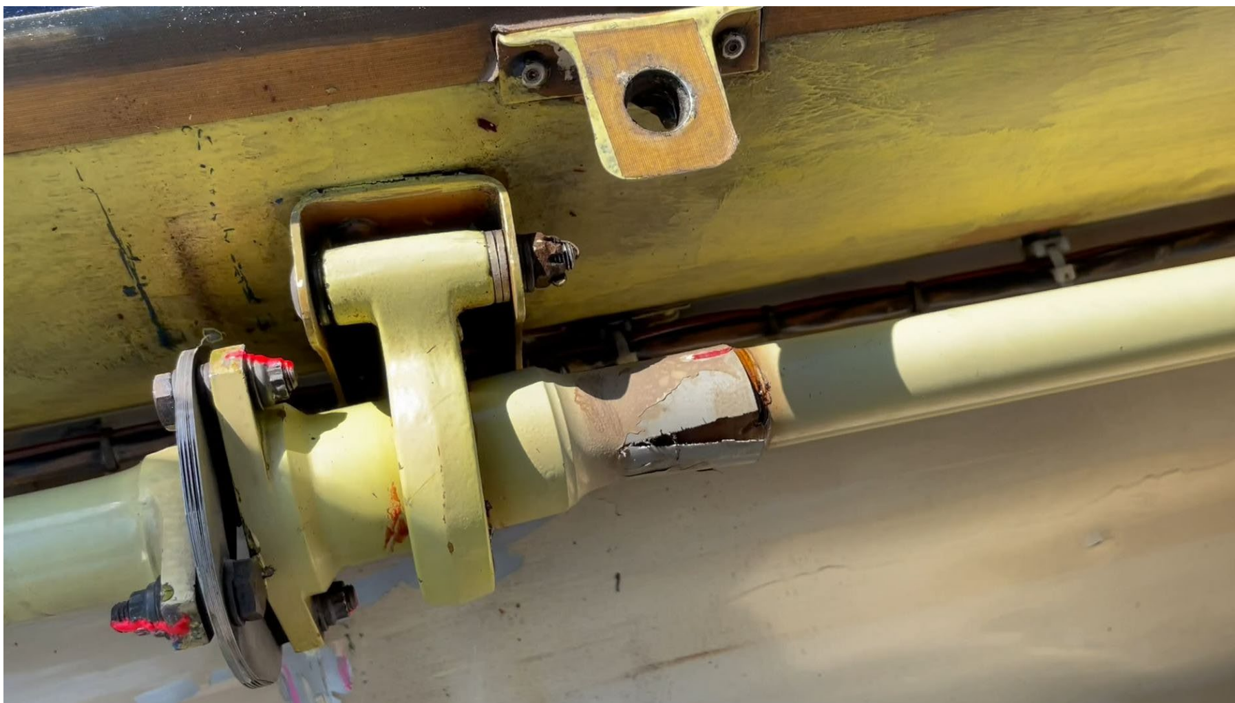
Photograph 2 - View of the tail rotor driveshaft (Courtesy of the FAA)
