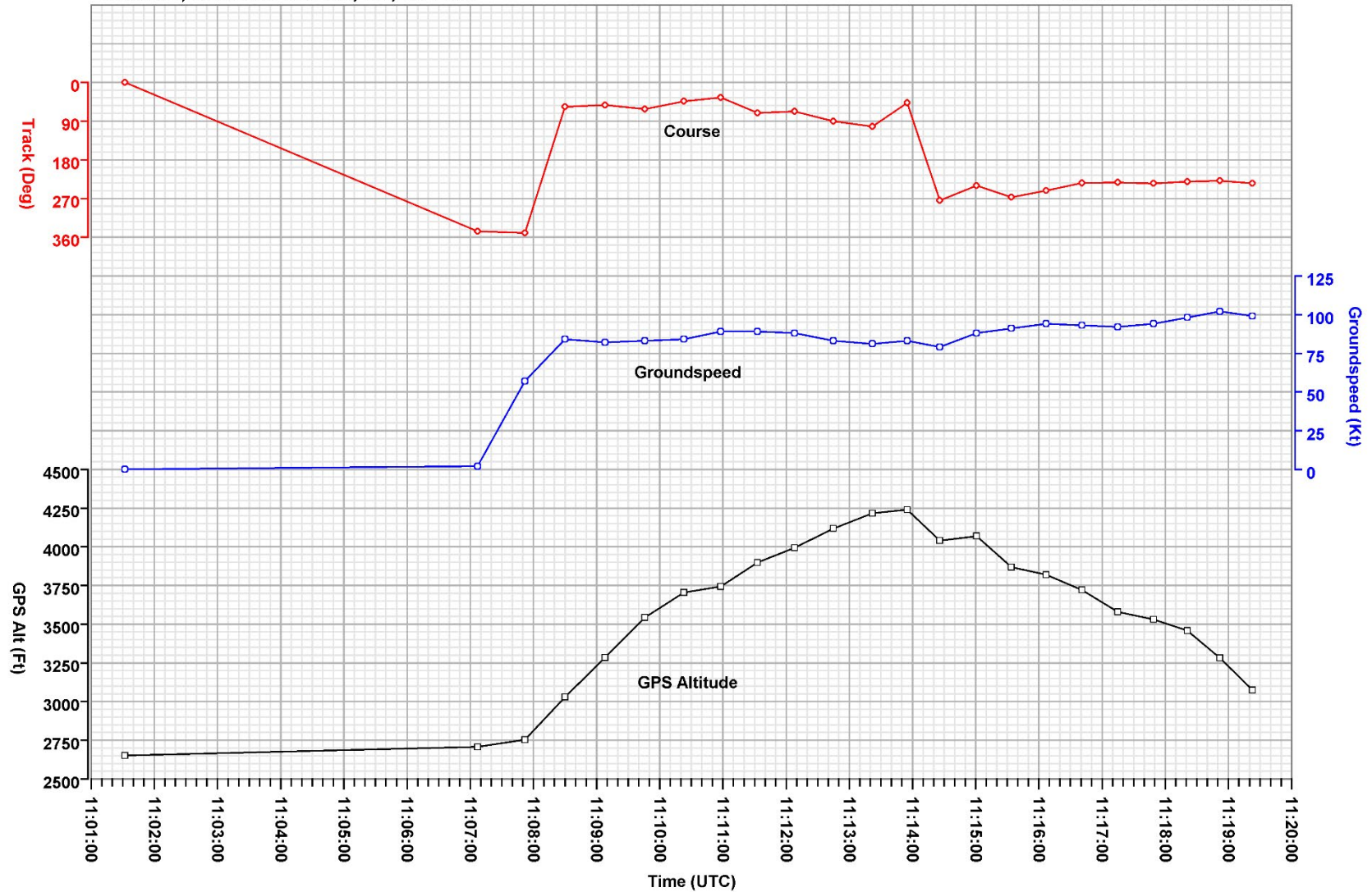
Plots of Garmin GPSMAP 296 parameters.
