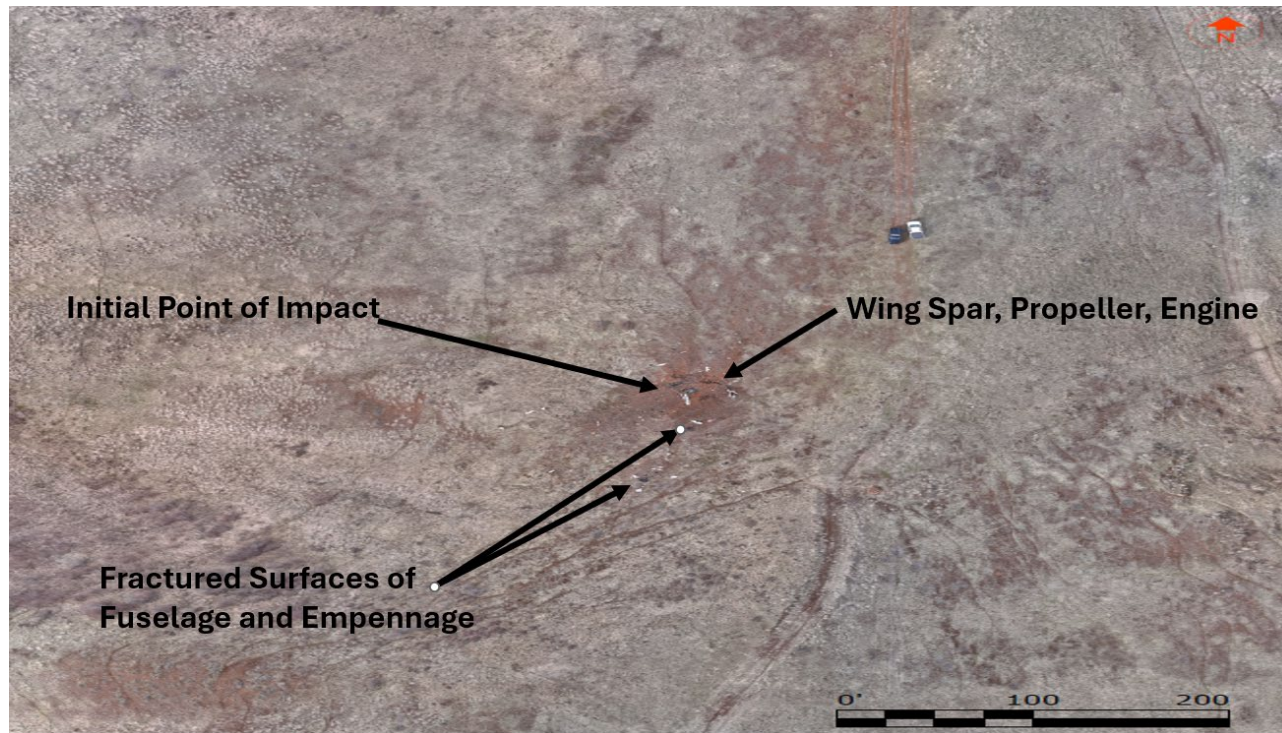
Photograph 1 - Aerial view of impact crater and main wreckage (Courtesy of LEA)
