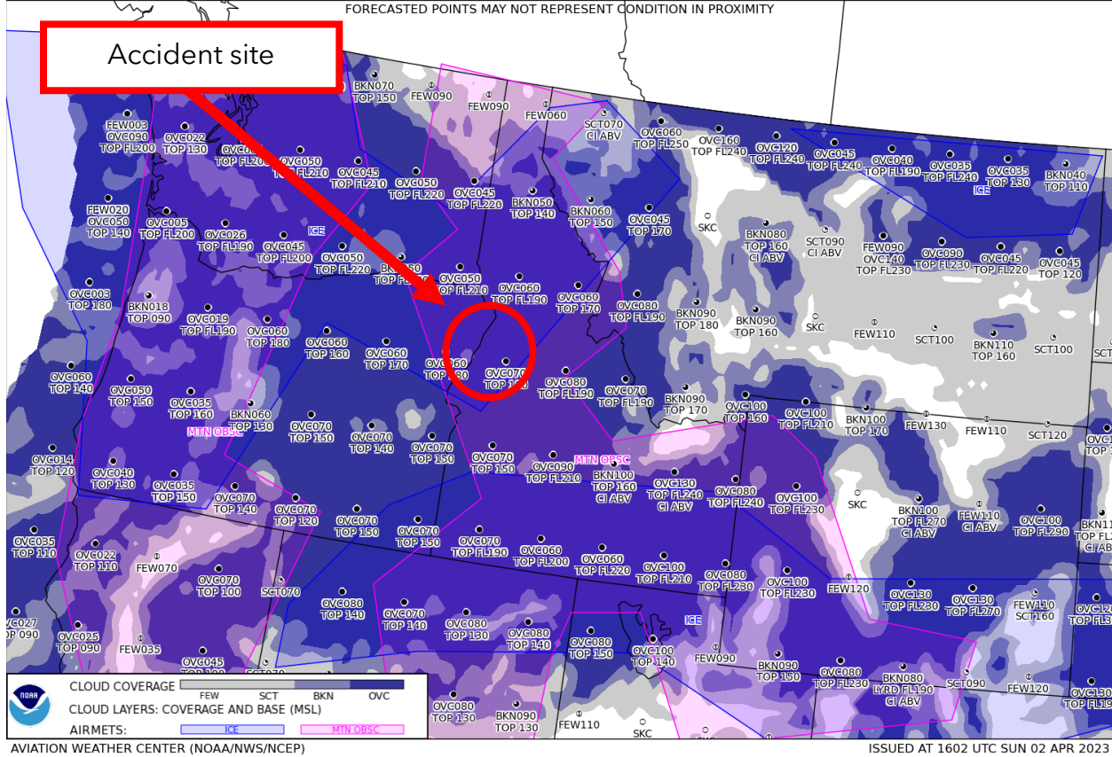
Figure 5. GFA Aviation Clouds Forecast valid at 1100 PDT with forecast issued at 0902 PDT.
