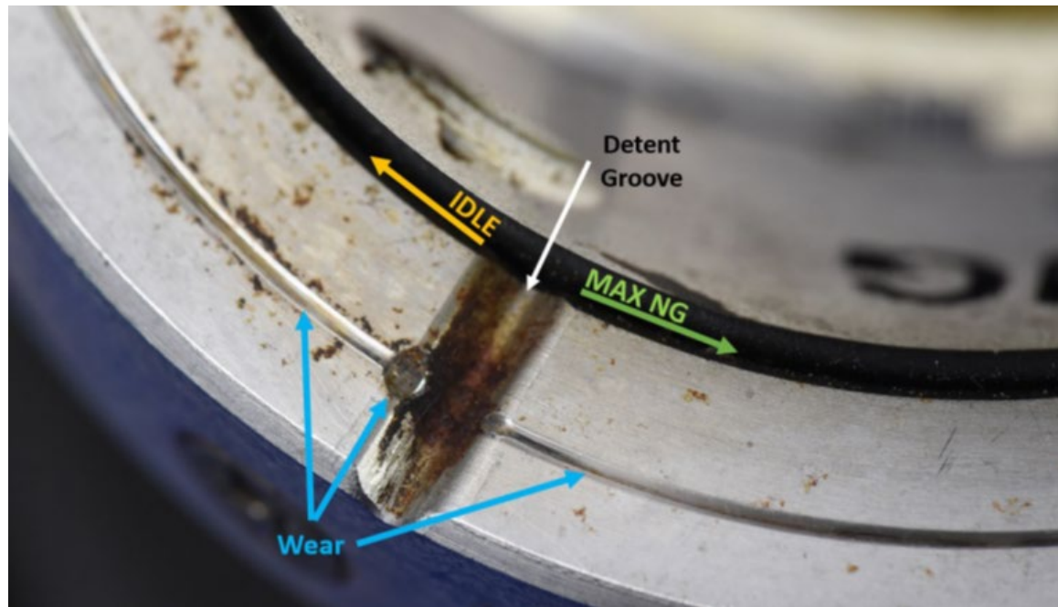
Photograph 5 - Throttle Detent Wear (Courtesy of Bell Helicopters)
