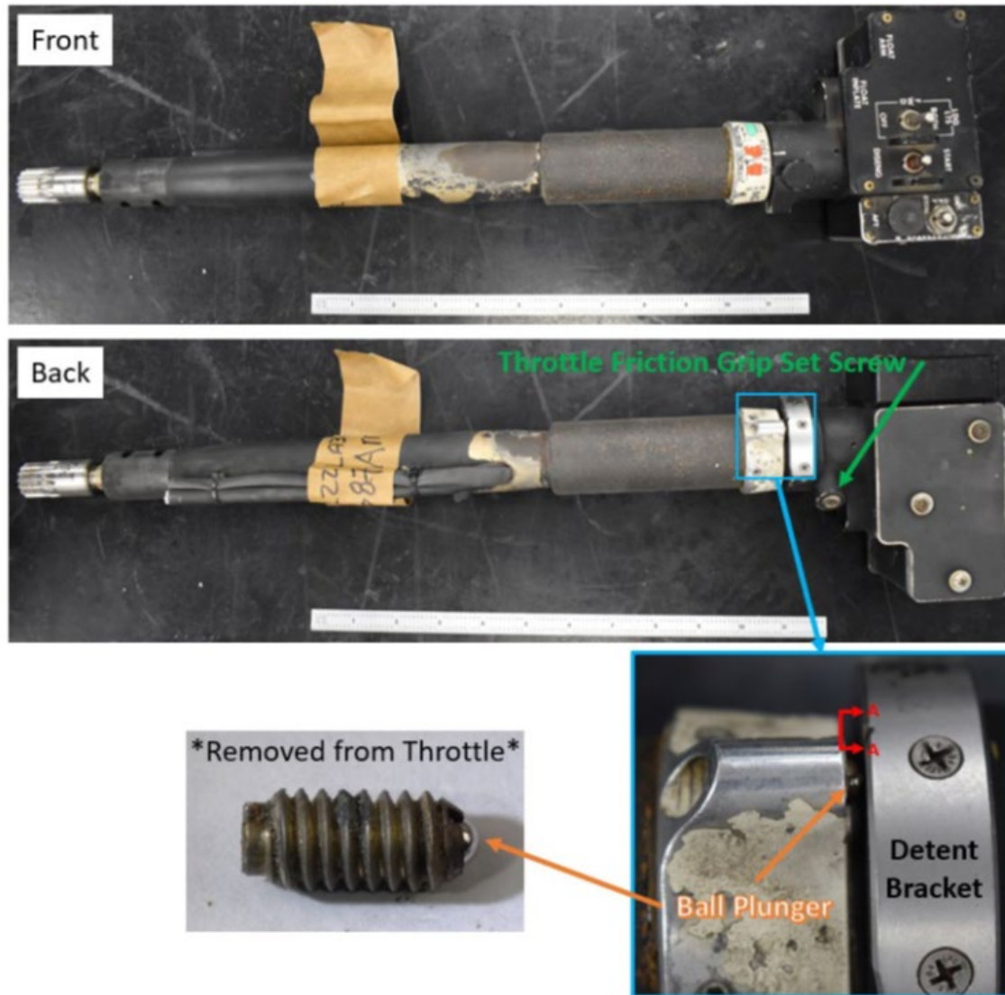
Photograph 4 - Collective Assembly and Throttle Components (Courtesy of Bell Helicopters)
