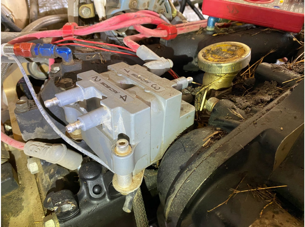
Figure 2. Coil pack. (Photo courtesy of the FAA)
